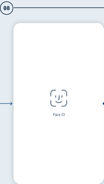
Operation authorization
