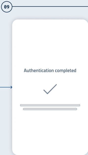
Authentication completed
