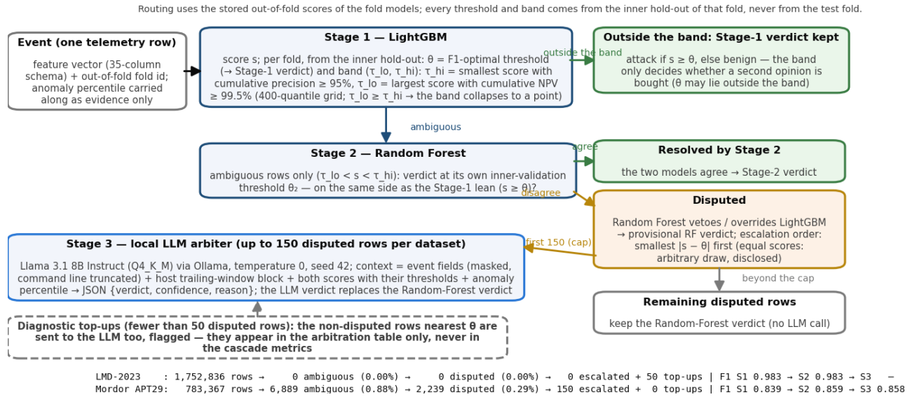
Figure 2. Software block diagram of the cascade and the LLM arbitration: accepted Stage-1 decisions, the ambiguous band, Random-Forest agreement and disputes, the escalation cap and the diagnostic top-ups; counts from the run.
