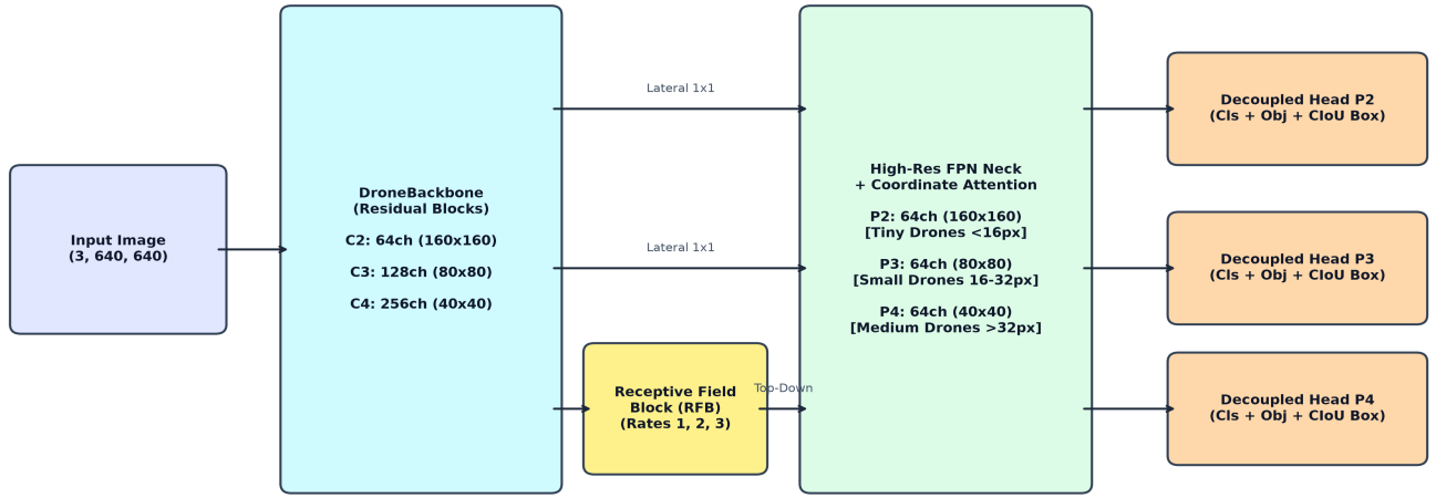
Fig. 1. Architecture of DroneNet-FPN-Attention: Backbone with RFB, High-Res FPN with Coordinate Attention, and Decoupled Detection Heads.
