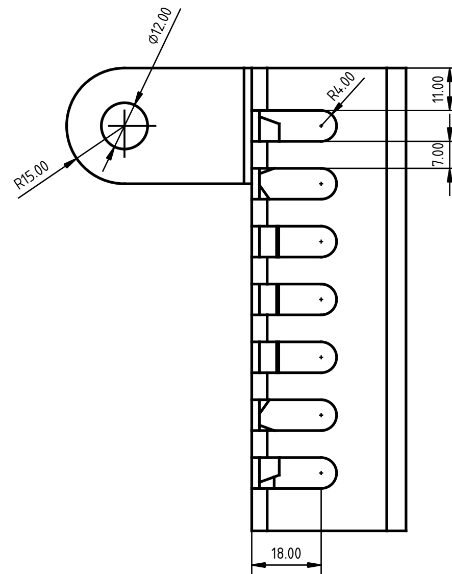
左側面図(LEFT SIDE VIEW)
