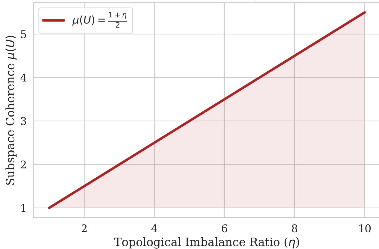
(a) The Statistical Front: Subspace Distortion
