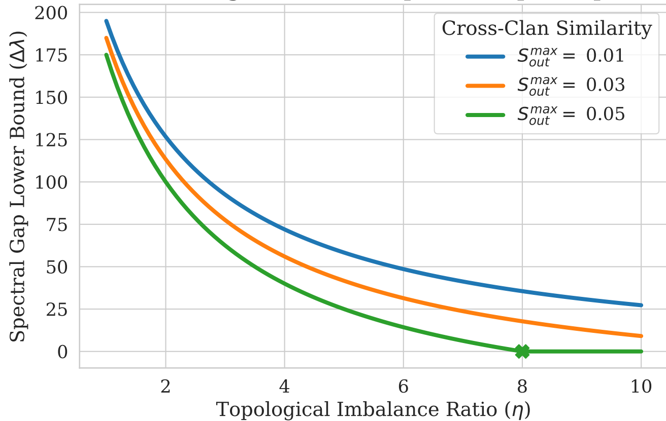
(b) The Algebraic Front: Spectral Gap Collapse
