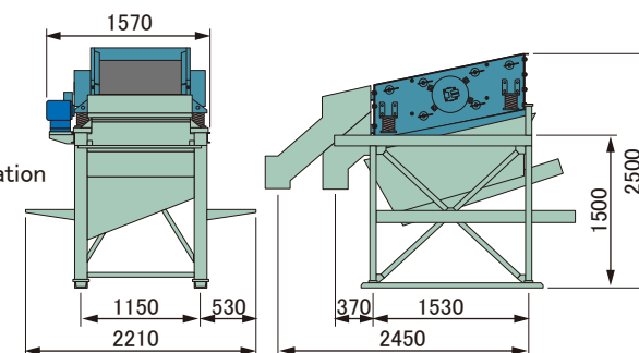
HV35F (Electric Type)
