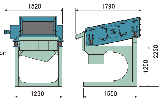
HVVH35E (Hydraulic Type)
