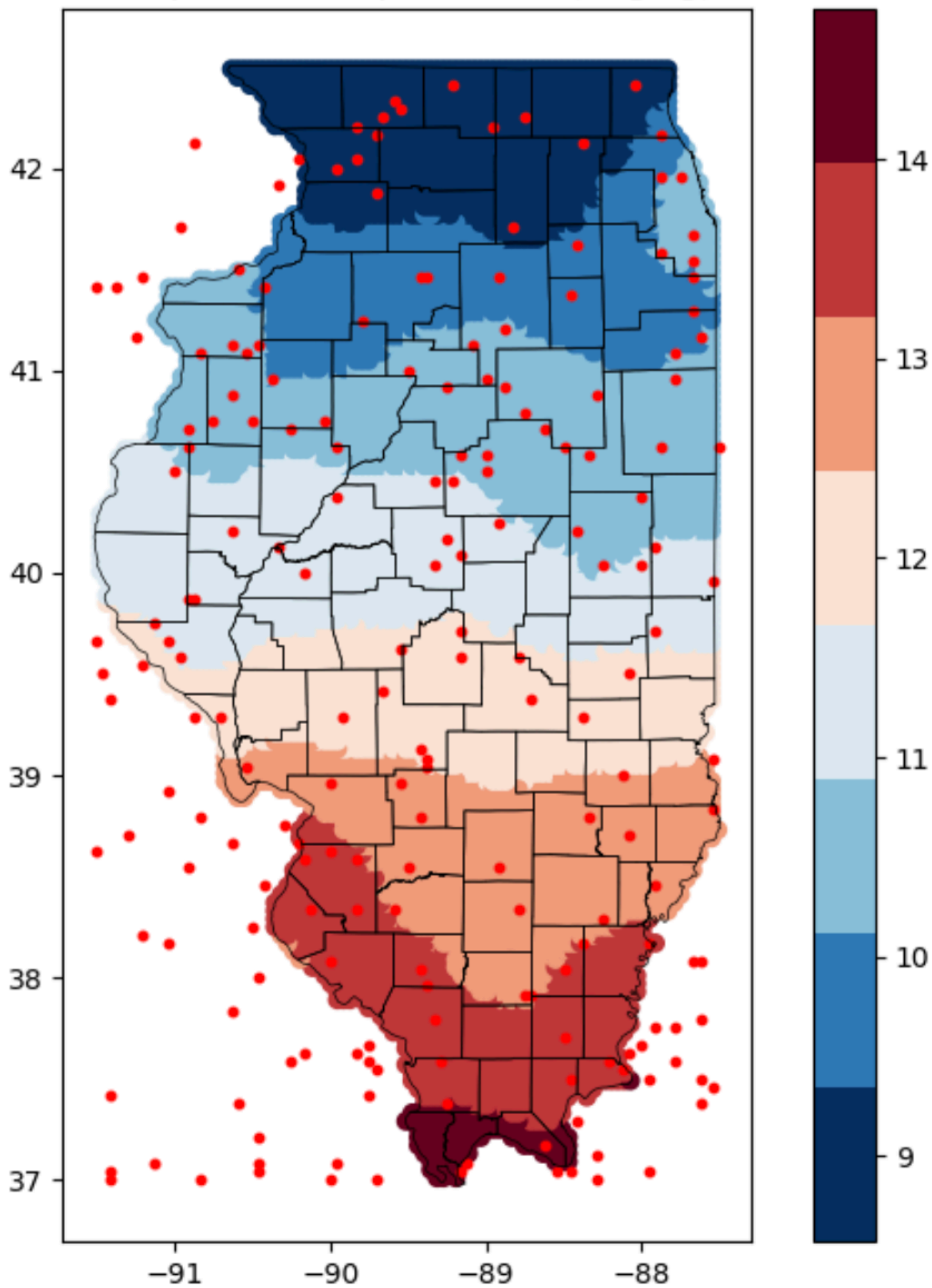
Temperature map of Illinois (Kriging)
