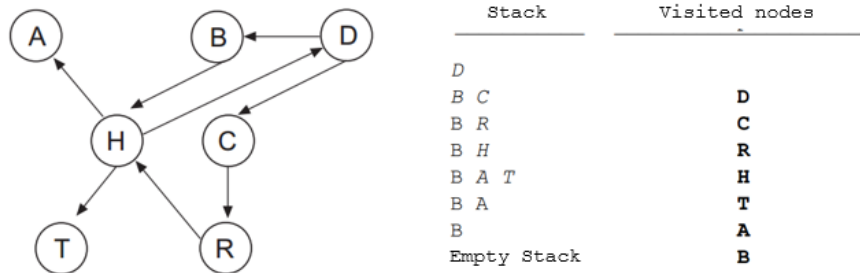
Figure 5.7: depth first
