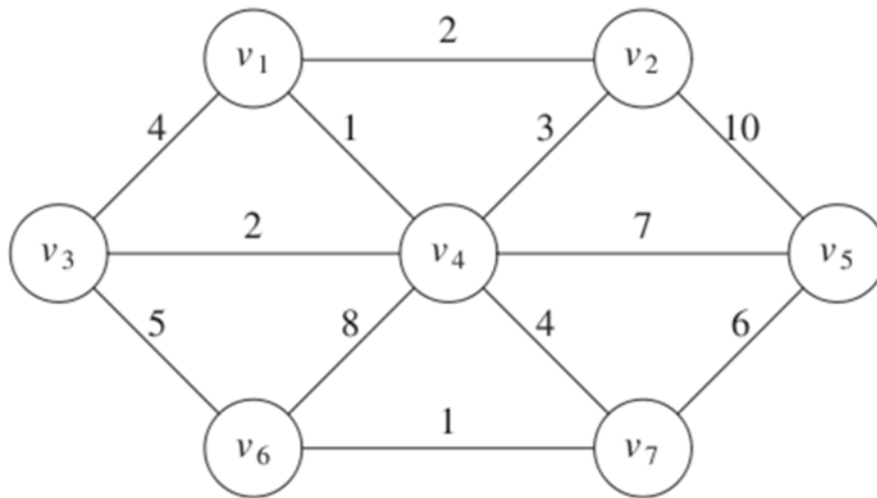
Figure 5.14: prim 1
