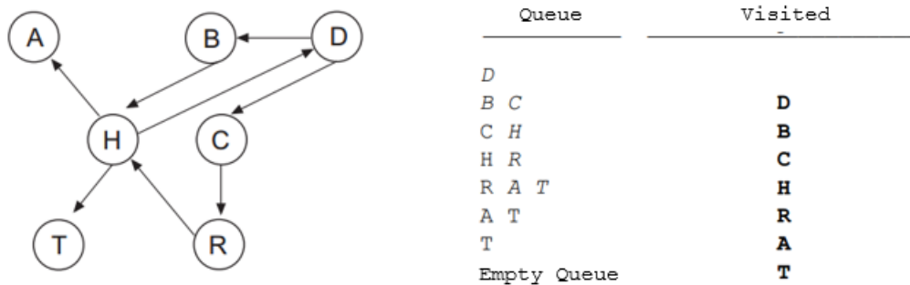
Figura 38: breadth first alg
