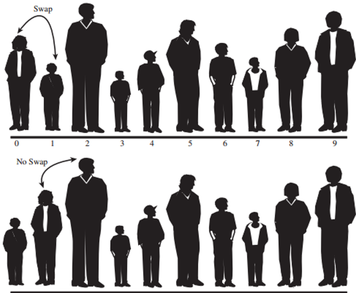
Figura 24: Bubble sort
