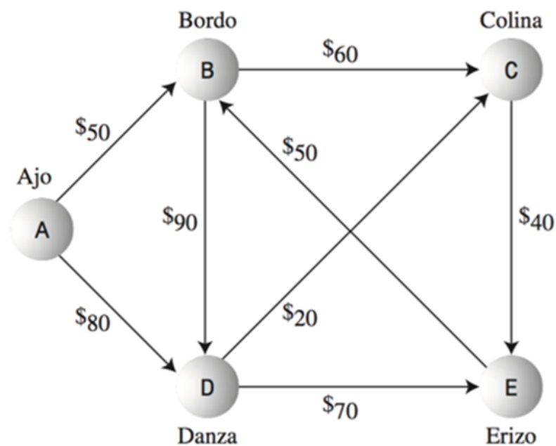
Figura 40: Dijkstra technique
