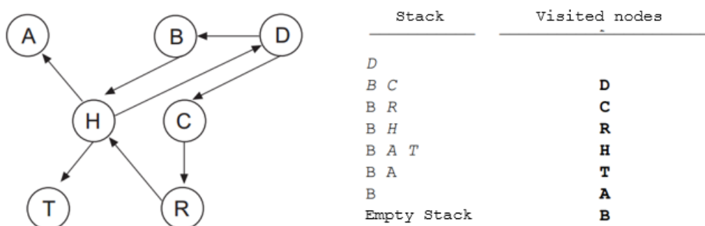
Figura 39: depth first
