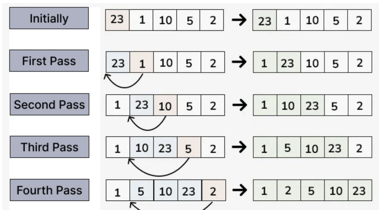
Figura 27: Insertion sort
