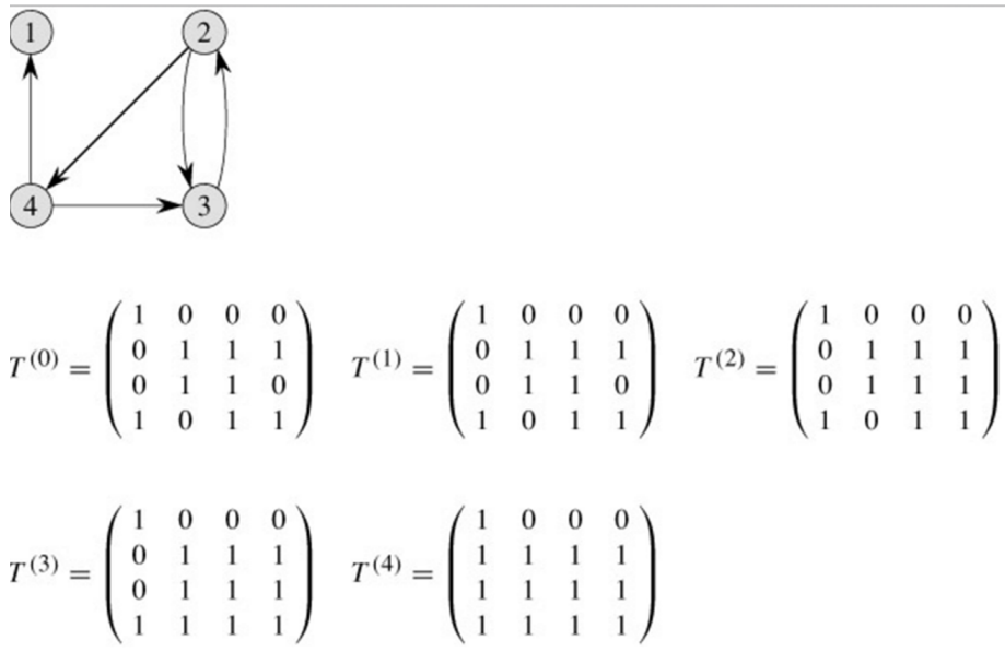
Figure 5.16: warshall algorithm2
