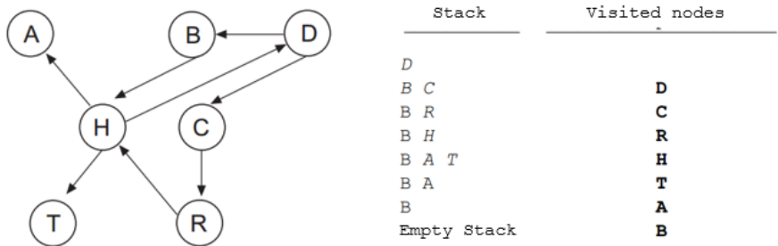
Figure 5.10: depth first
