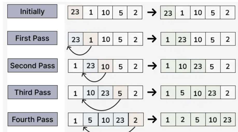
Figure 4.6: Insertion sort
