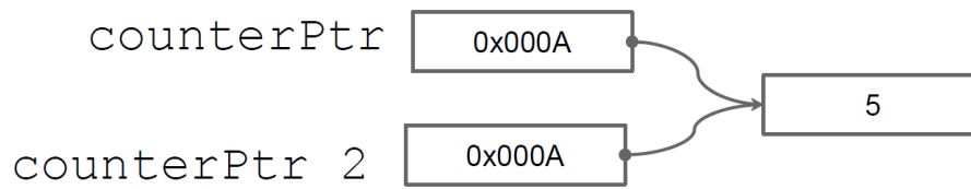
Figure 1.15: Shallow copy
