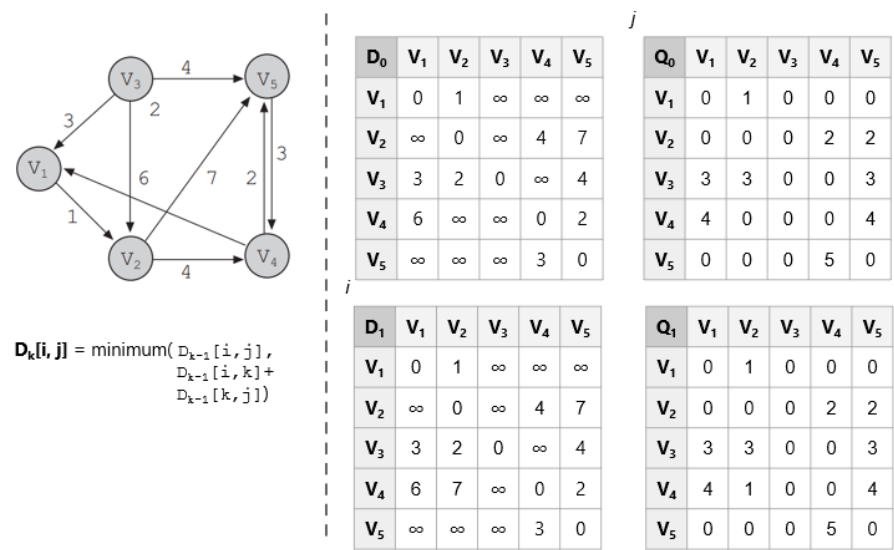
Figure 5.11: Floyd alg
