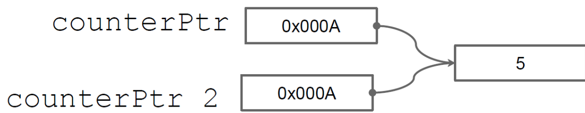
Figura 15: Shallow copy
