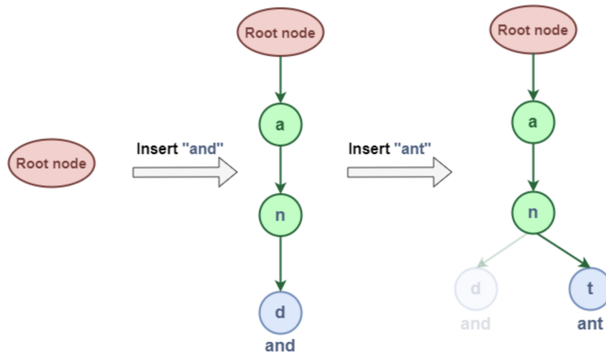
Figure 3.16: Trie
