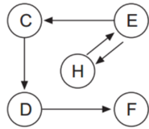
Directed graph
