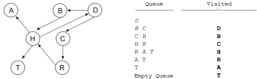
Figure 5.9: breadth first alg
