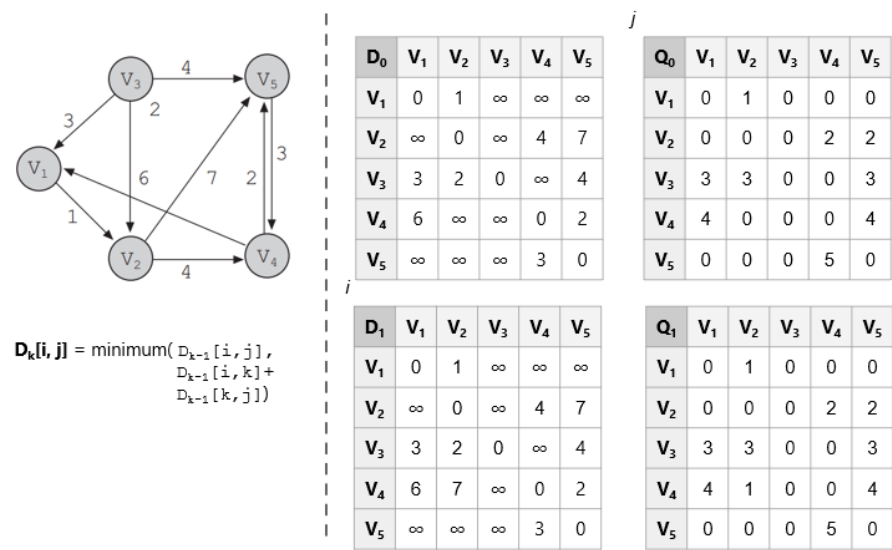
Figure 5.11: Floyd alg
