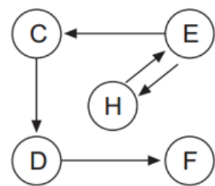
Directed graph
