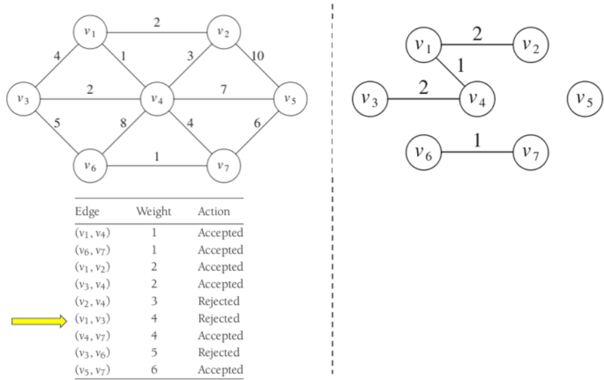
Figure 5.18: Kruskal
