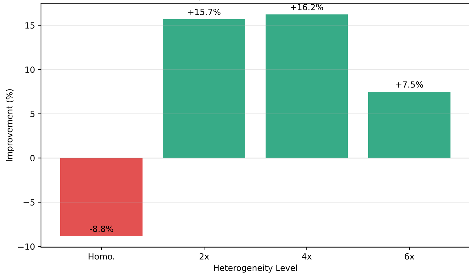
MPC Improvement Over Baseline PO2
