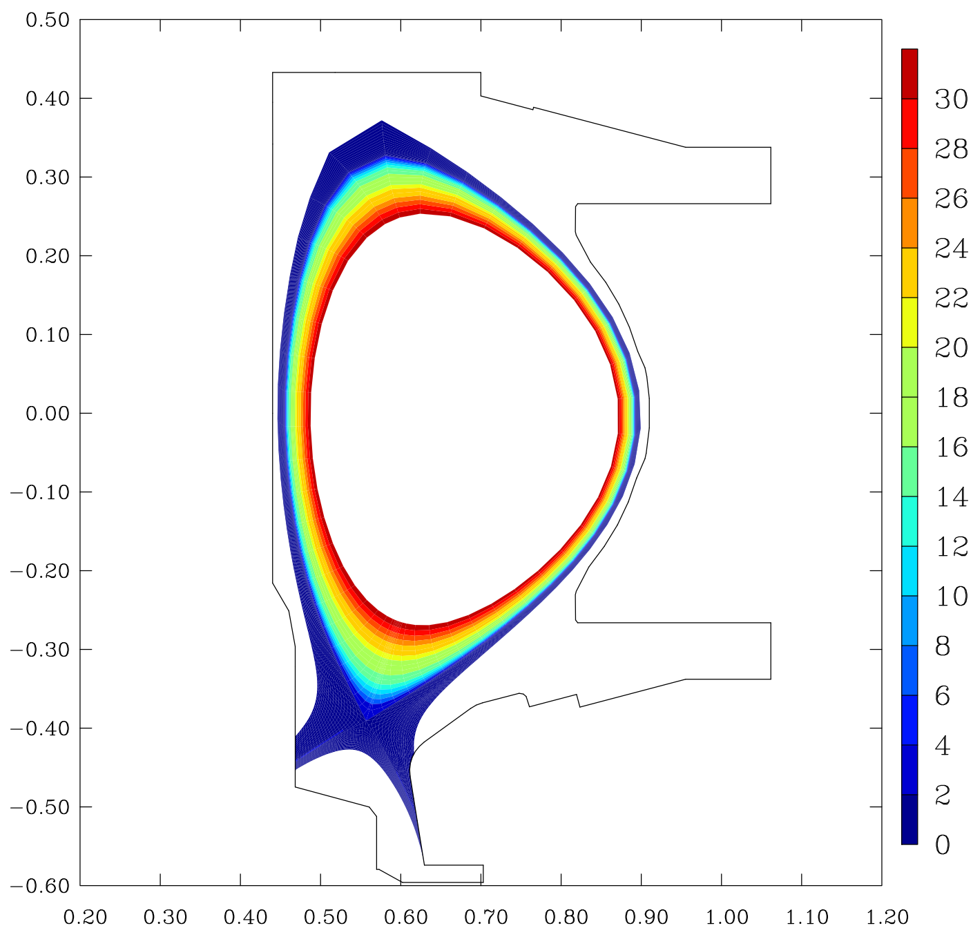
Electron Static Pressure [kPa]
