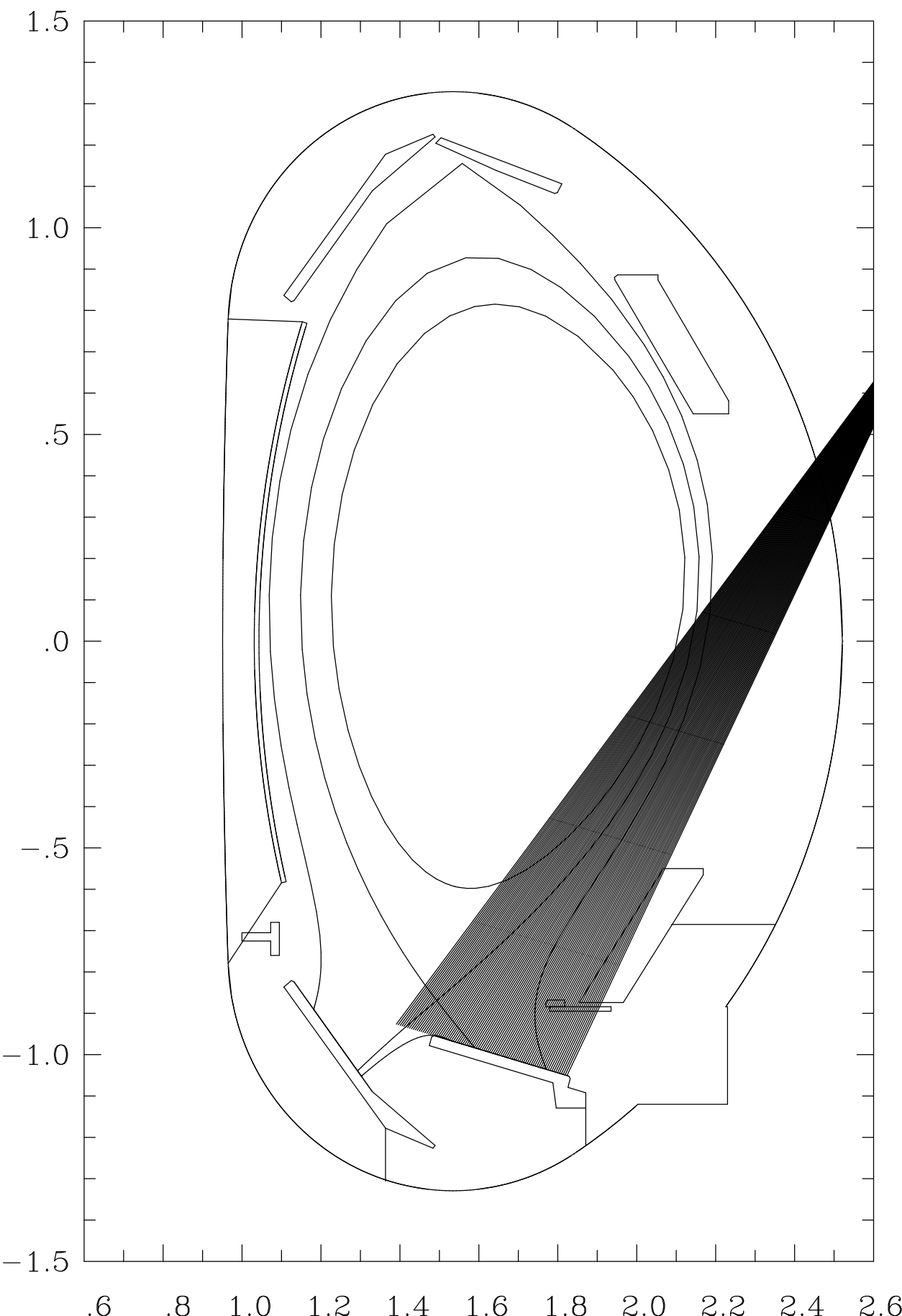
Boundary Layer Spectrometer
