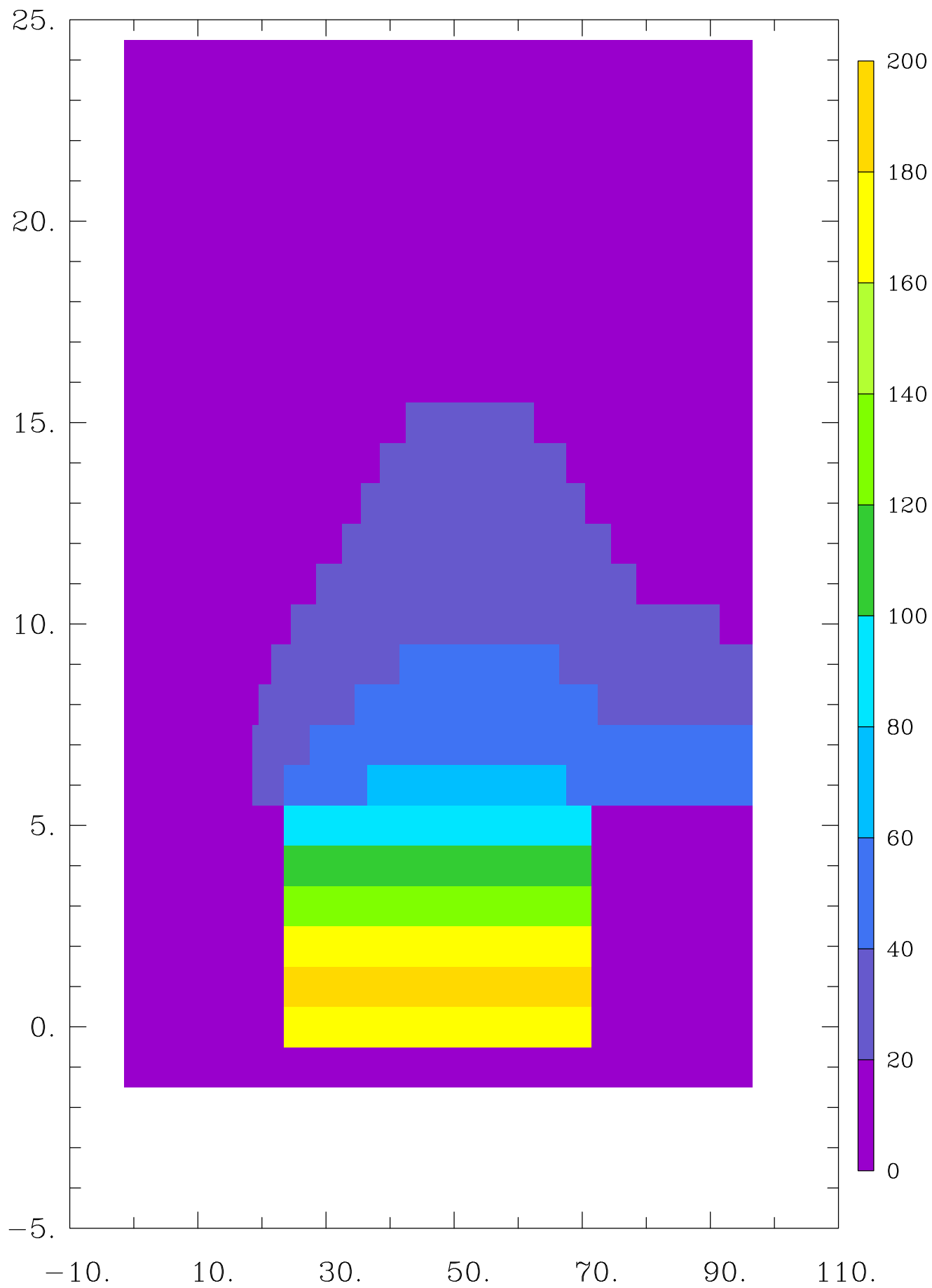
Electron temperature (eV)
