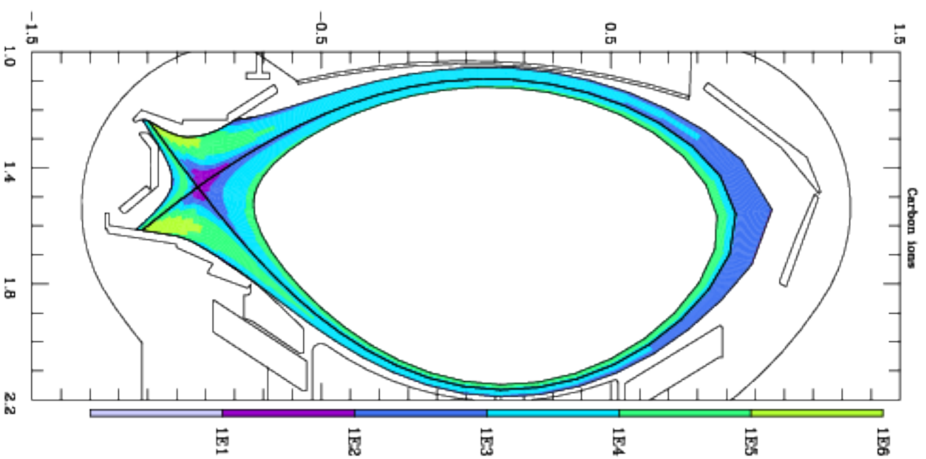
Total radiation loss (W/m 2 ) Carbon ions
