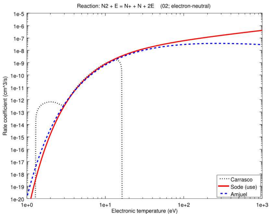
Figure 3 : Comparison of different rate coefficient data for ionization of \text{N}_2 by electron impact
