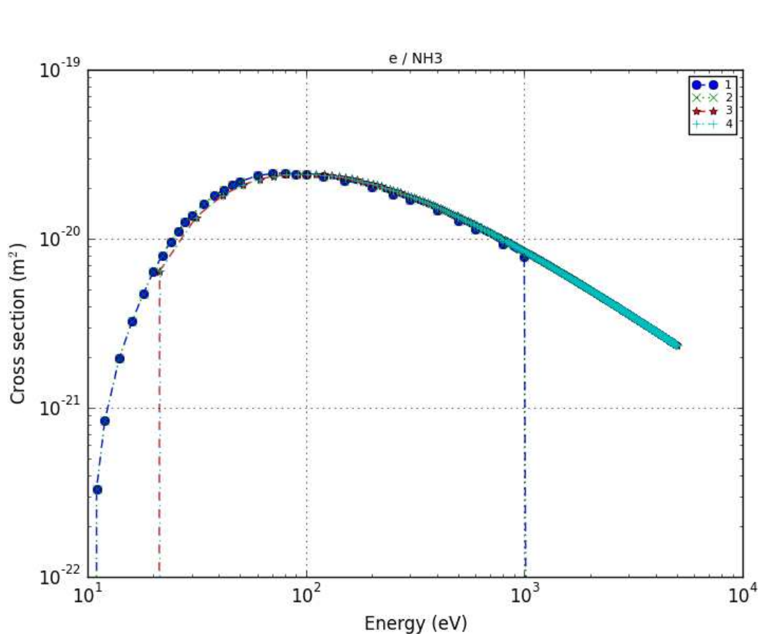
Figure 1 : Comparison between different sources cited in Lxcat Hayashi database (1), Morgan database (2), Quantemol database (3&4) for cross section in \text{NH}_3 ionization processes
