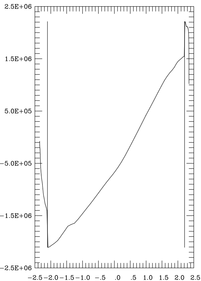
parallel ion energy flux (W) SUMY &lt;iy = 19&gt;
