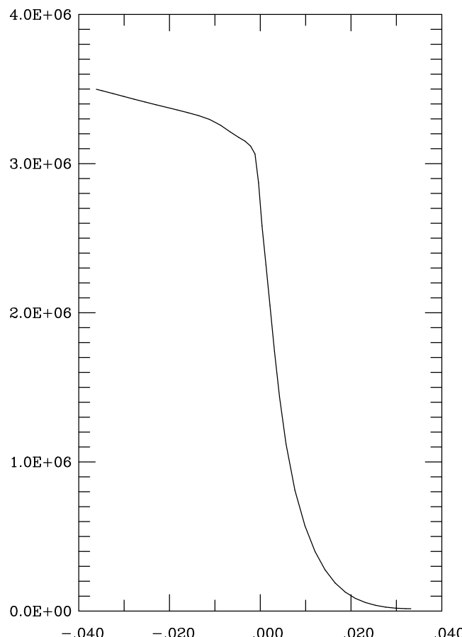
perpendicular ion energy flux (W) SUMX &lt;ix = 57&gt;
