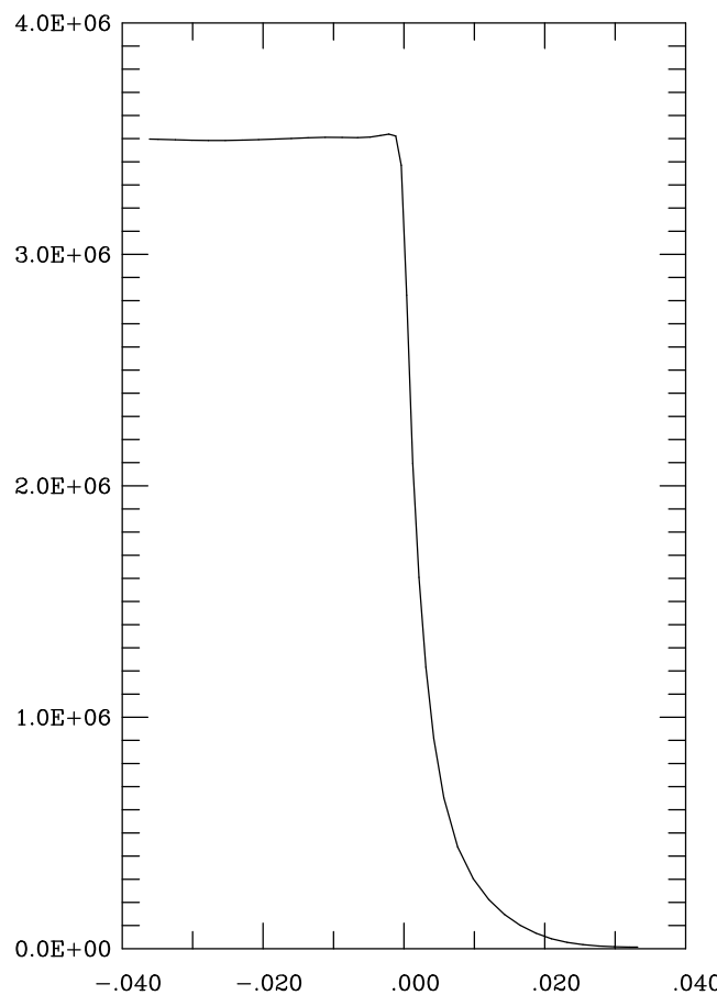
perpendicular ion energy flux (W) SUMX &lt;ix = 57&gt;
