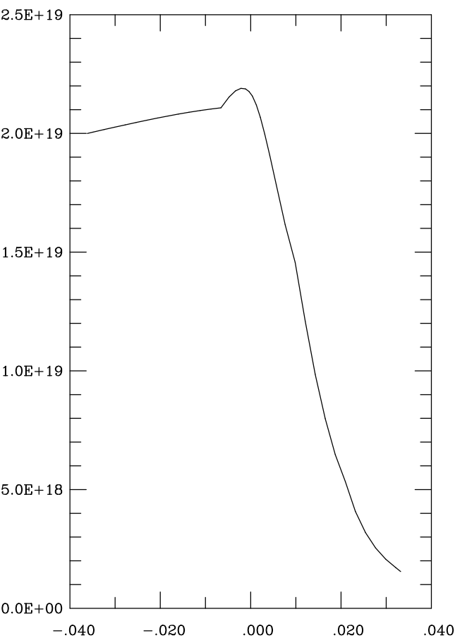
Ion density (m -3 ) SUM Ne1+ to Ne10+ <ix = 57>
