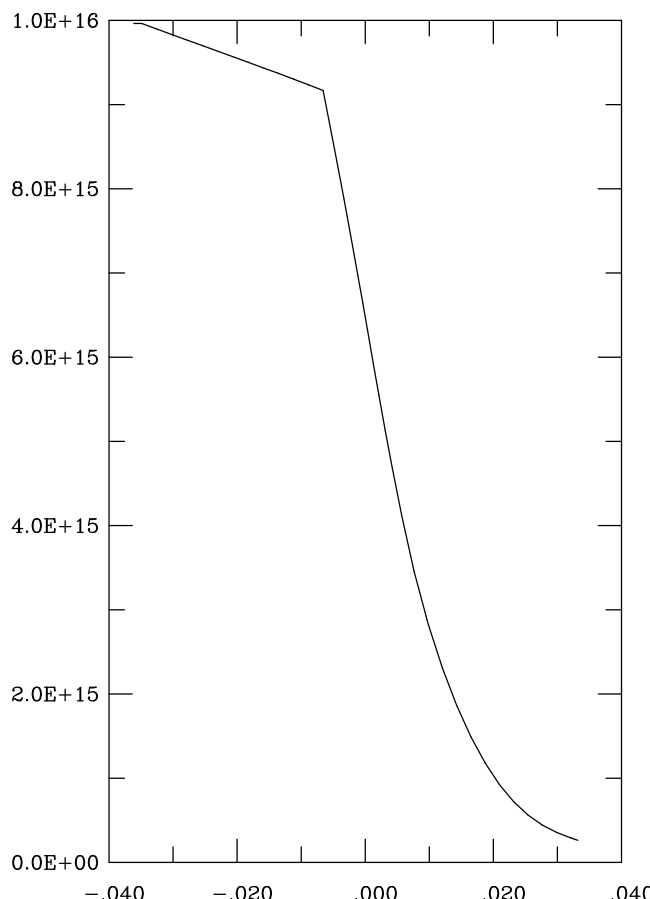
Ion density (m -3 ) SUM He1+ to He2+ <ix = 57>
