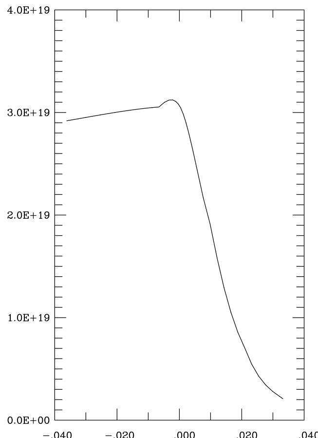
electron density (m -3 ) <ix = 57>
