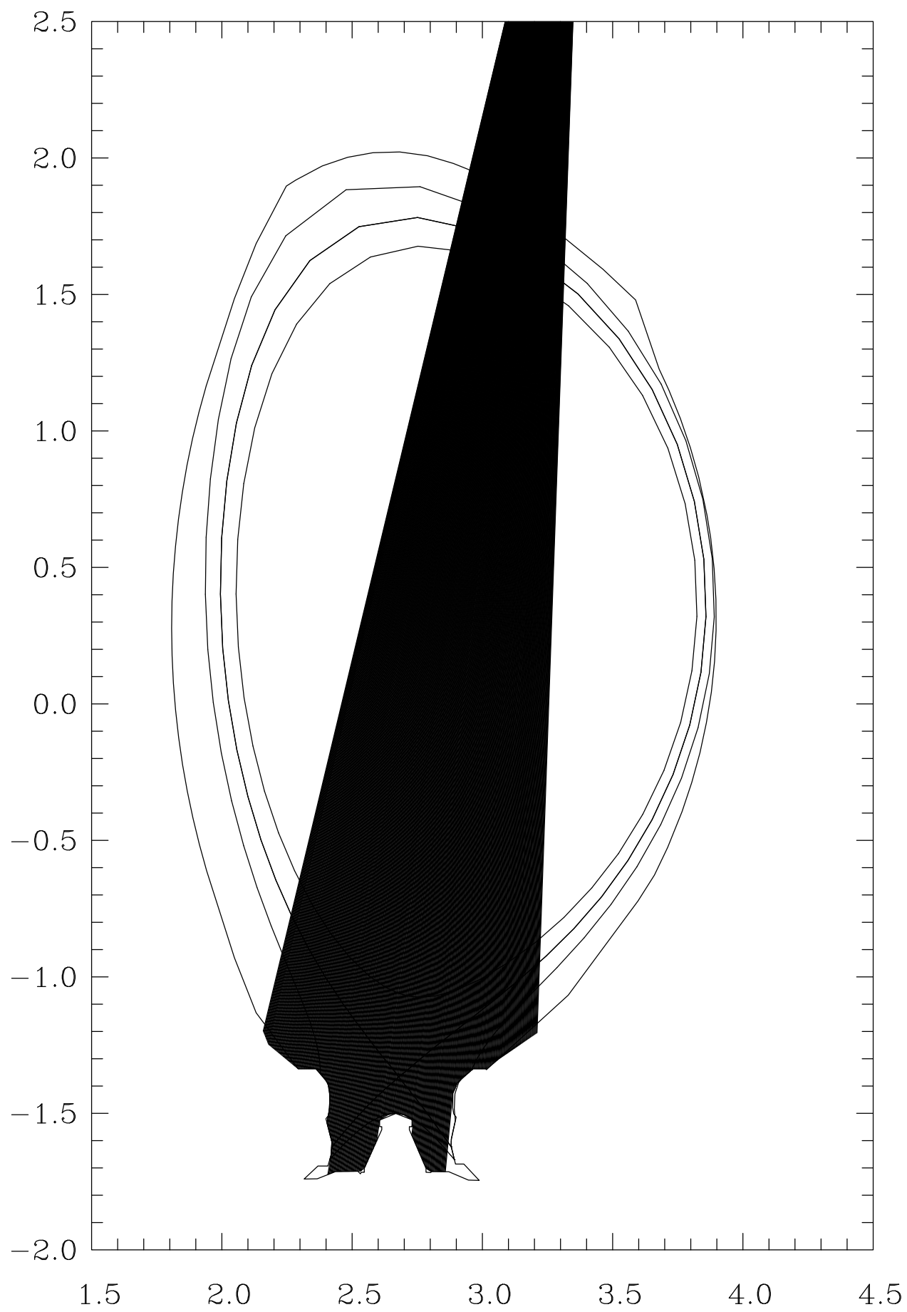
KL2 chords
