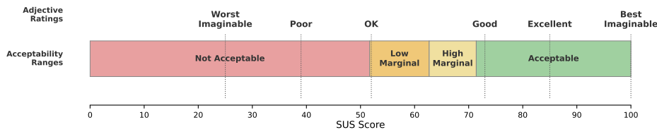
Figure 6.2: SUS score interpretation framework showing adjective ratings and acceptability ranges. Adapted from Bangor, Kortum, and Miller [83].
