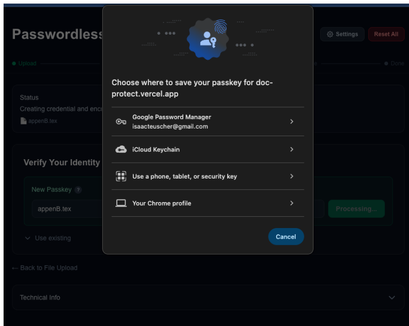
Figure 5.4: Save-a-passkey prompts presented by the user's passkey provider during credential creation.
