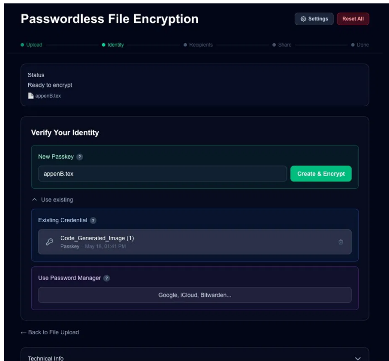
Figure 5.2: Identity verification step with new passkey option and create and encrypt action.
