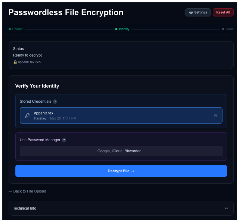
Figure 5.7: Decryption identity step with decrypt file action.
