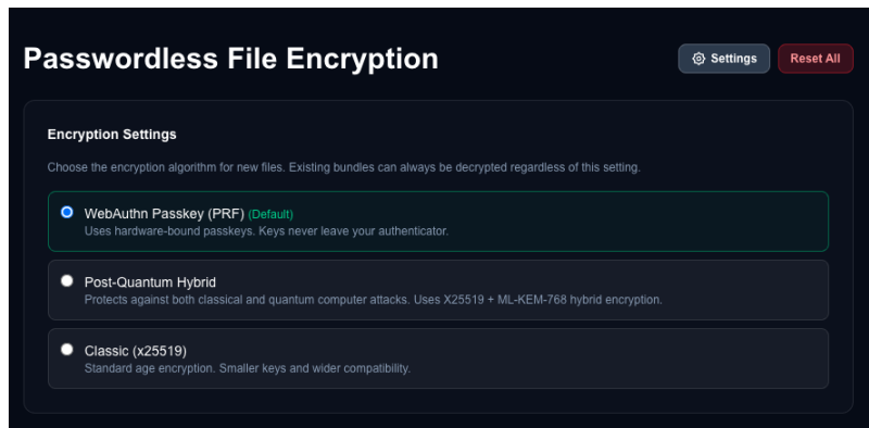
Figure 5.8: Settings panel with encryption algorithm selection.
