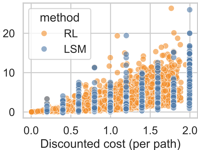
Path-level discounted reward vs cost
