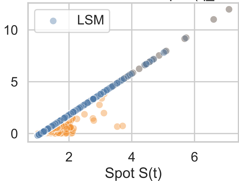
Discounted reward vs spot ( q_t > 0 )
