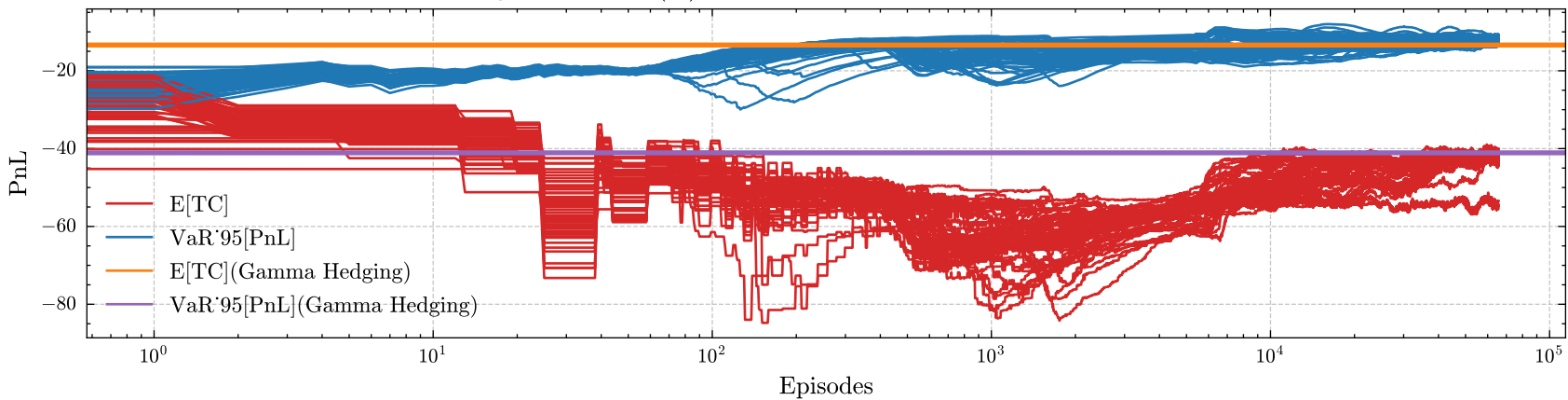
Rolling Mean PnL(T) per episode trained - CVaR - Spread 2%
