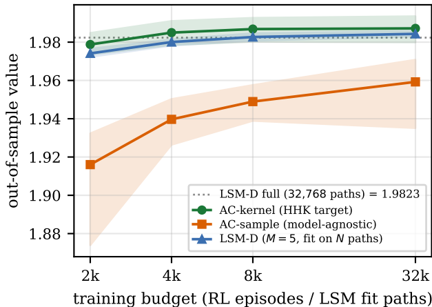
Sample efficiency at the focal cell ( c = 0.04 , \gamma_c = 2 )
