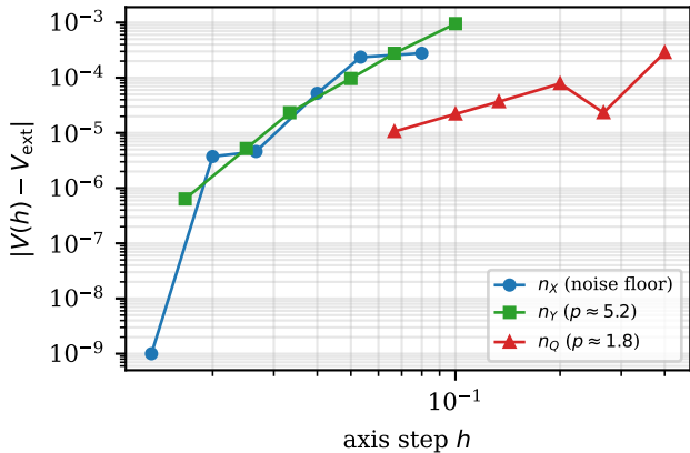
(a) Grid convergence, focal cell
