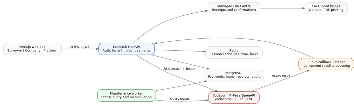
Figure 1 - LoanHub M-Pesa runtime architecture
