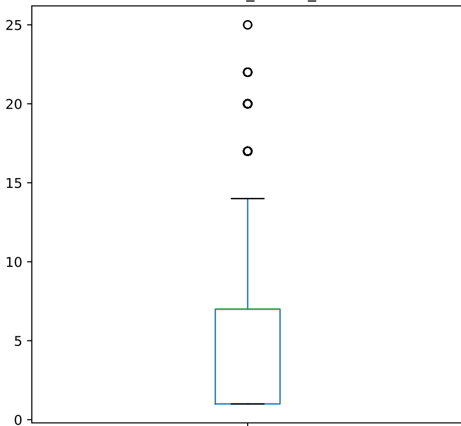
admission_source_id
