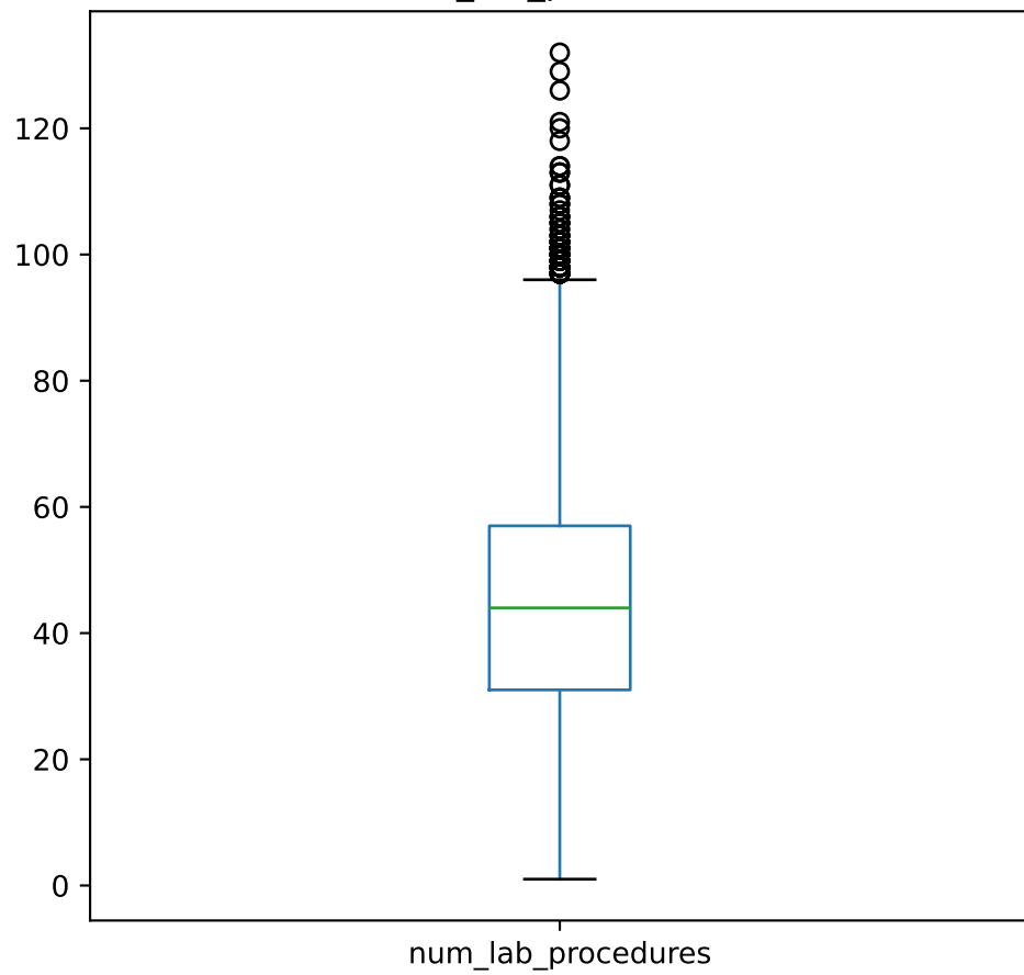
num_lab_procedures
