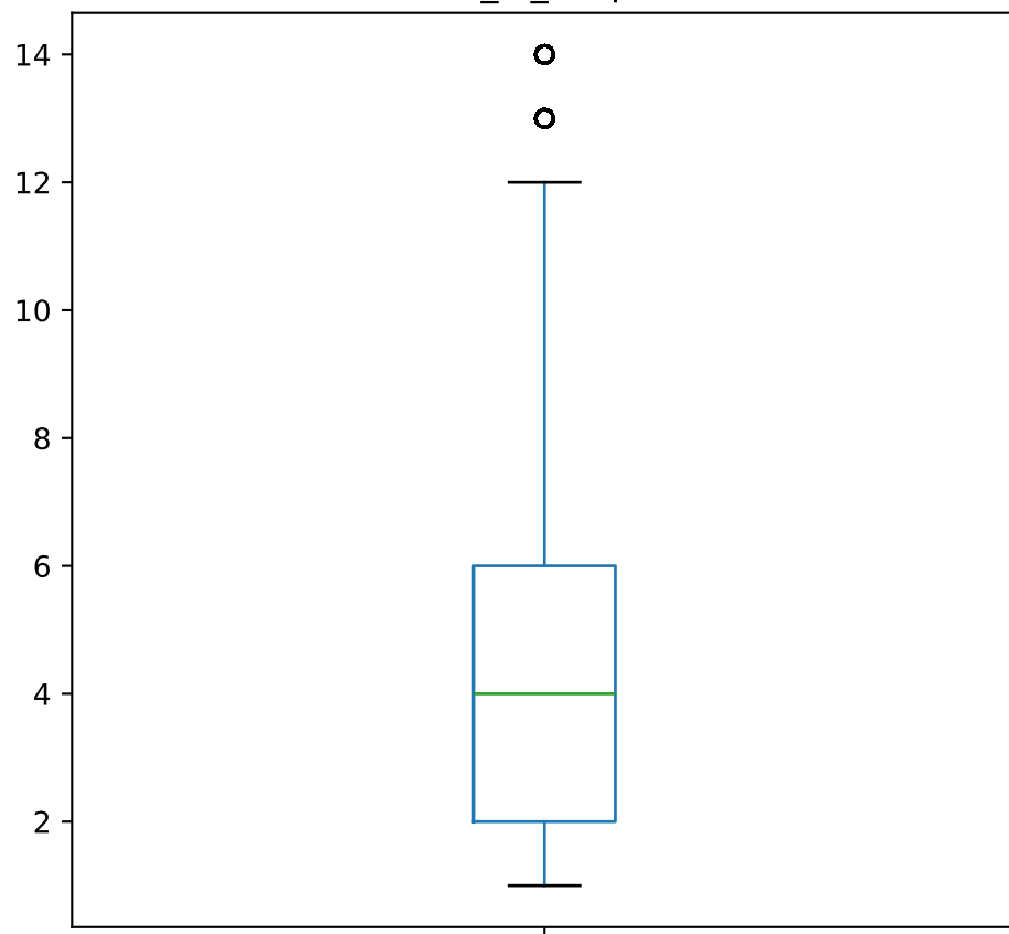
time_in_hospital
