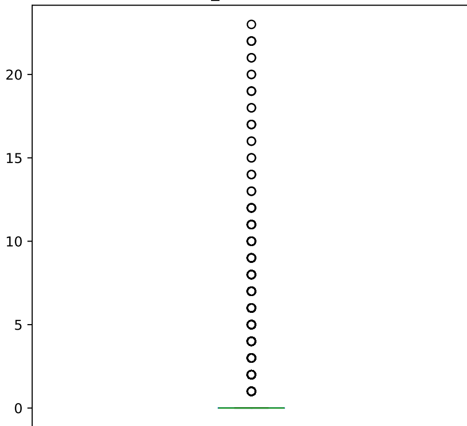
cum_readmissions
