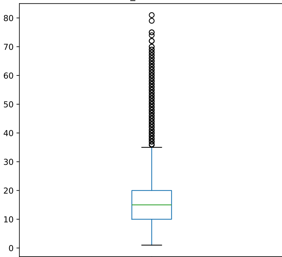
num_medications
