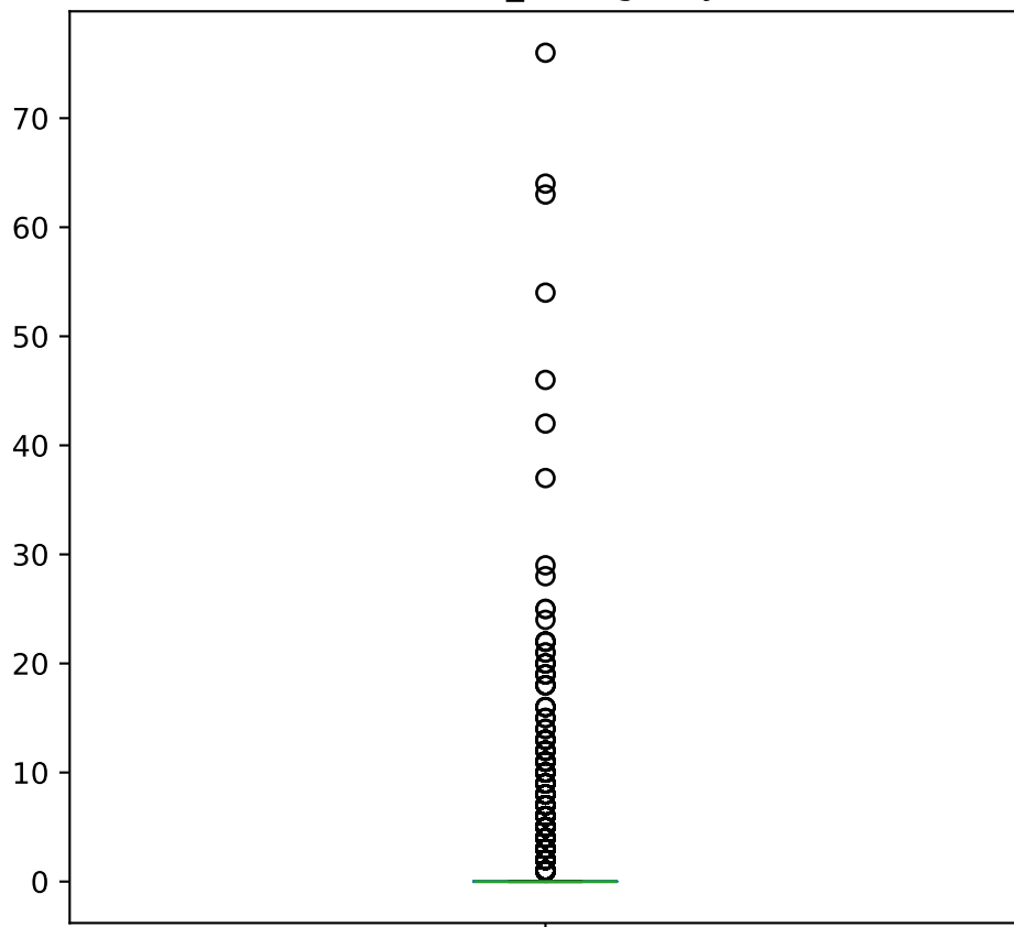
number_emergency
