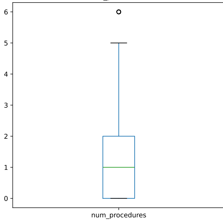
num_procedures
