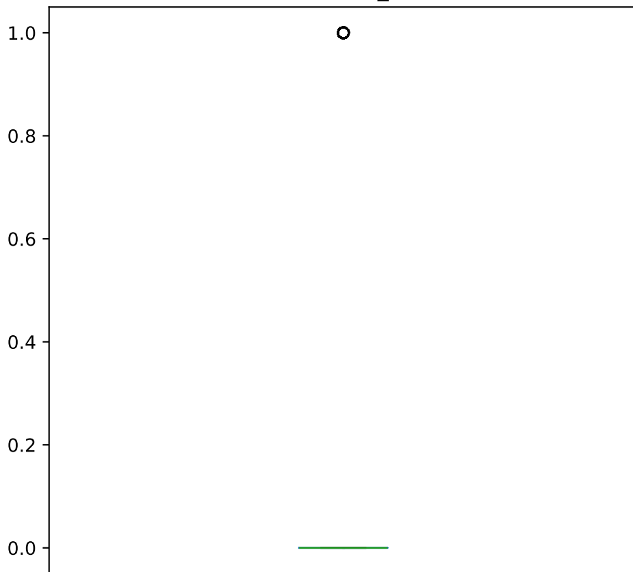
readmitted_30d
