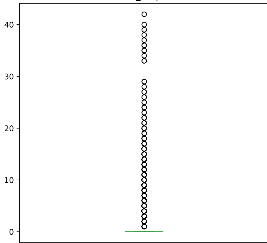
number_outpatient
