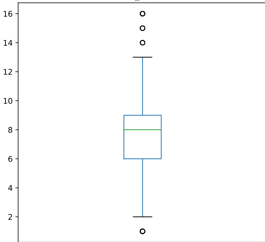
number_diagnoses
