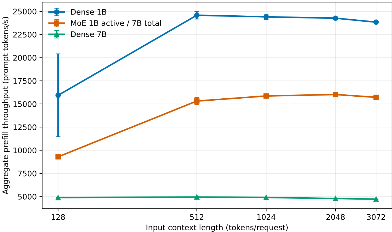
Prefill-dominated serving
