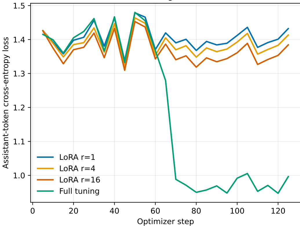
Training loss
