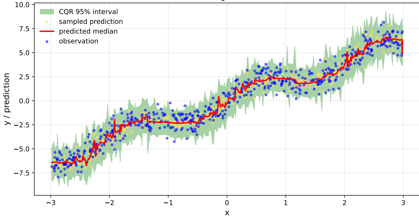
Conformal Quantile Regression (Random Forest)
