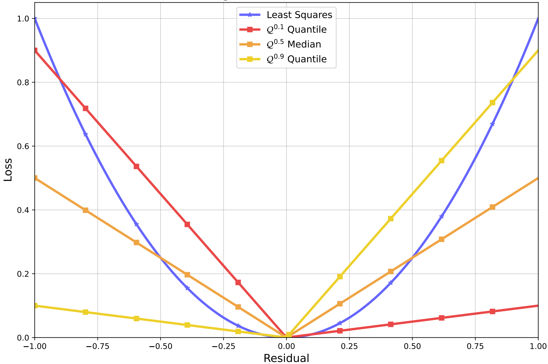
Regression: Loss Function
