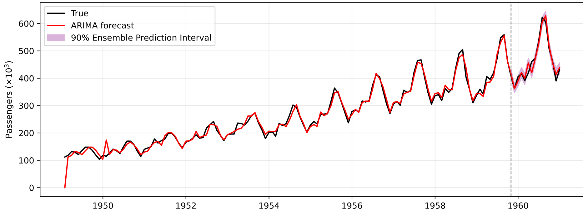
ARIMA + Residual Bootstrap Ensemble (90% PI)
