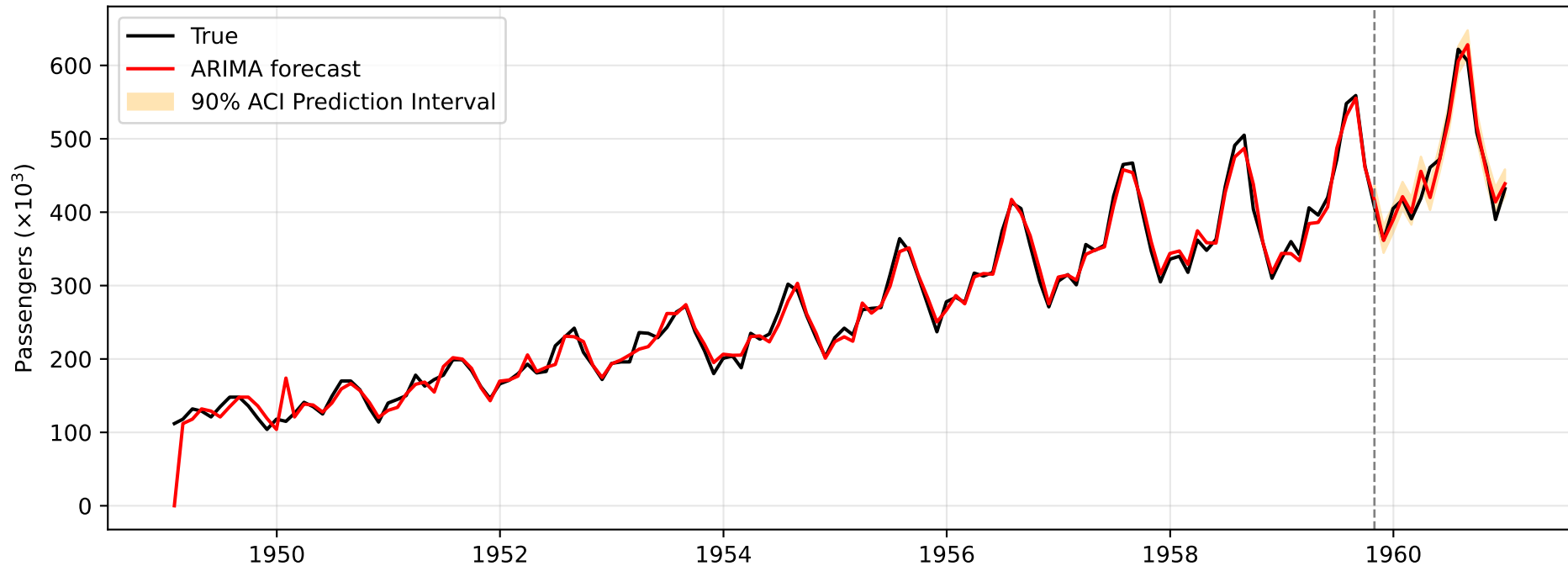
ARIMA + ACI-CQR (Adaptive 90% Prediction Interval)
