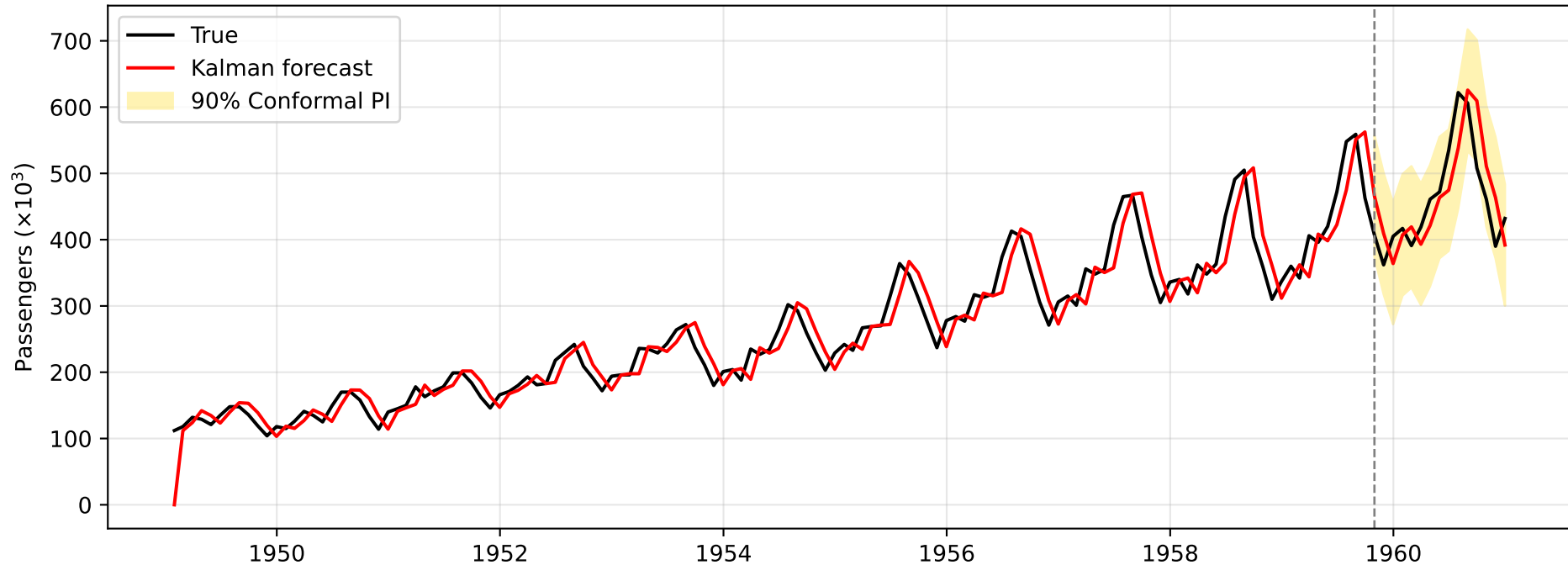
Kalman + Split Conformal (90% Prediction Interval)
