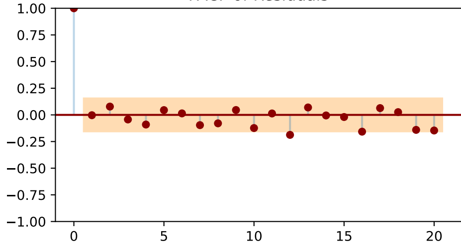
PACF of Residuals
