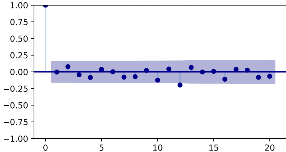
ACF of Residuals
