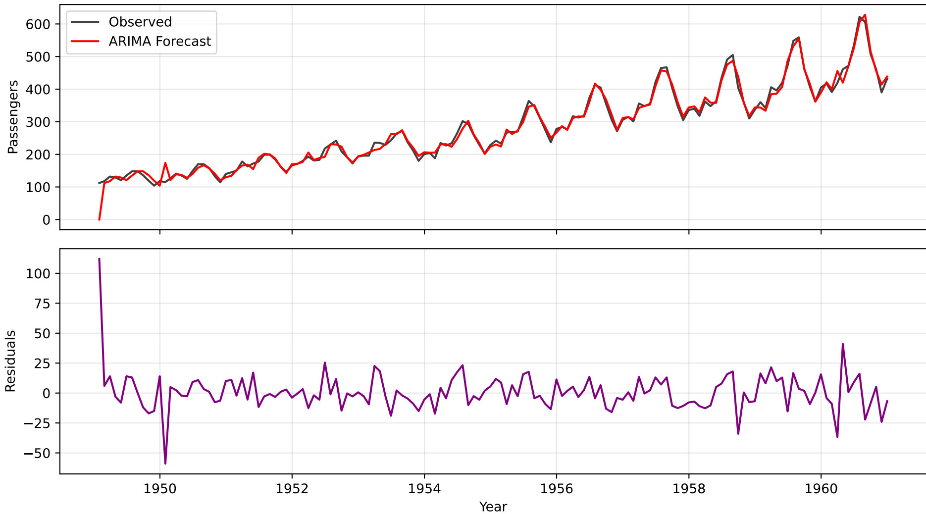
ARIMA Fit and Residuals
