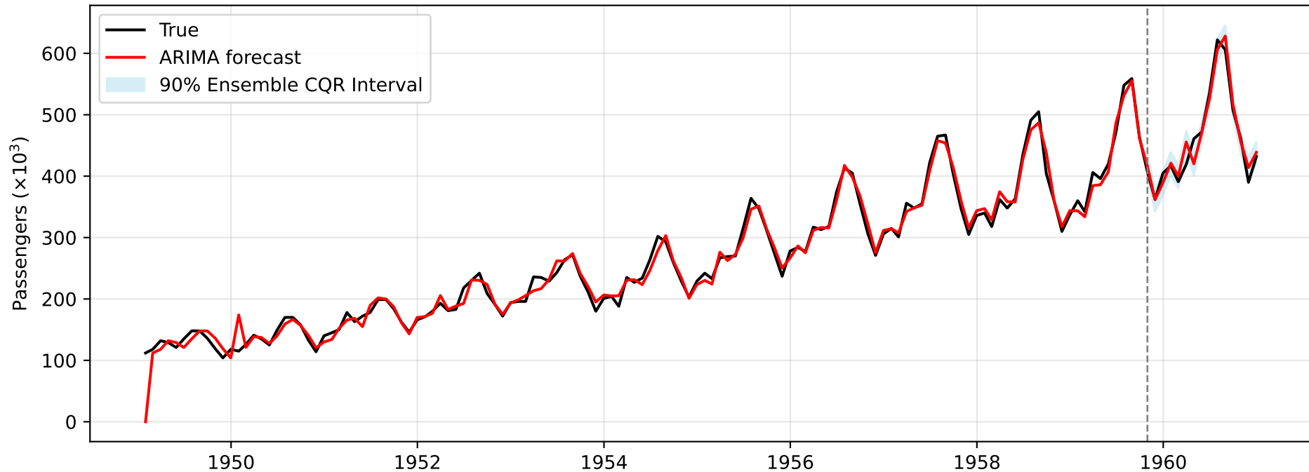
ARIMA + Ensemble CQR (90% Prediction Interval)
