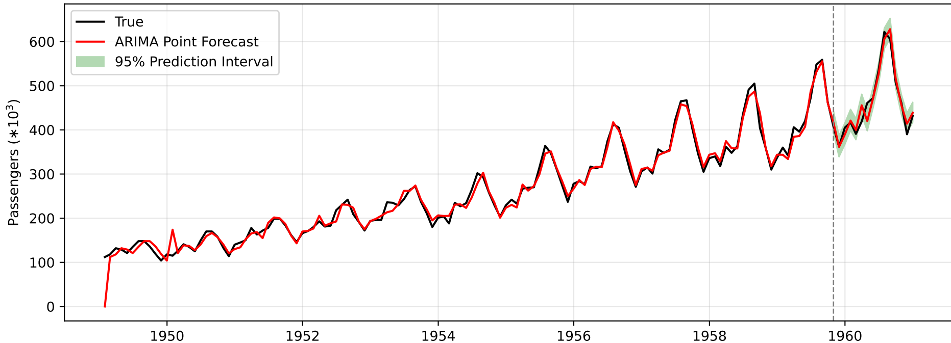
ARIMA + CQR: Uncertainty Quantification for Time Series
