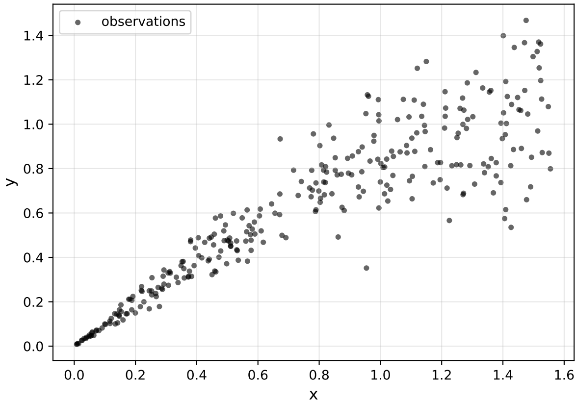
Heteroscedastic Regression: y = \sin(x) + \varepsilon(x)
