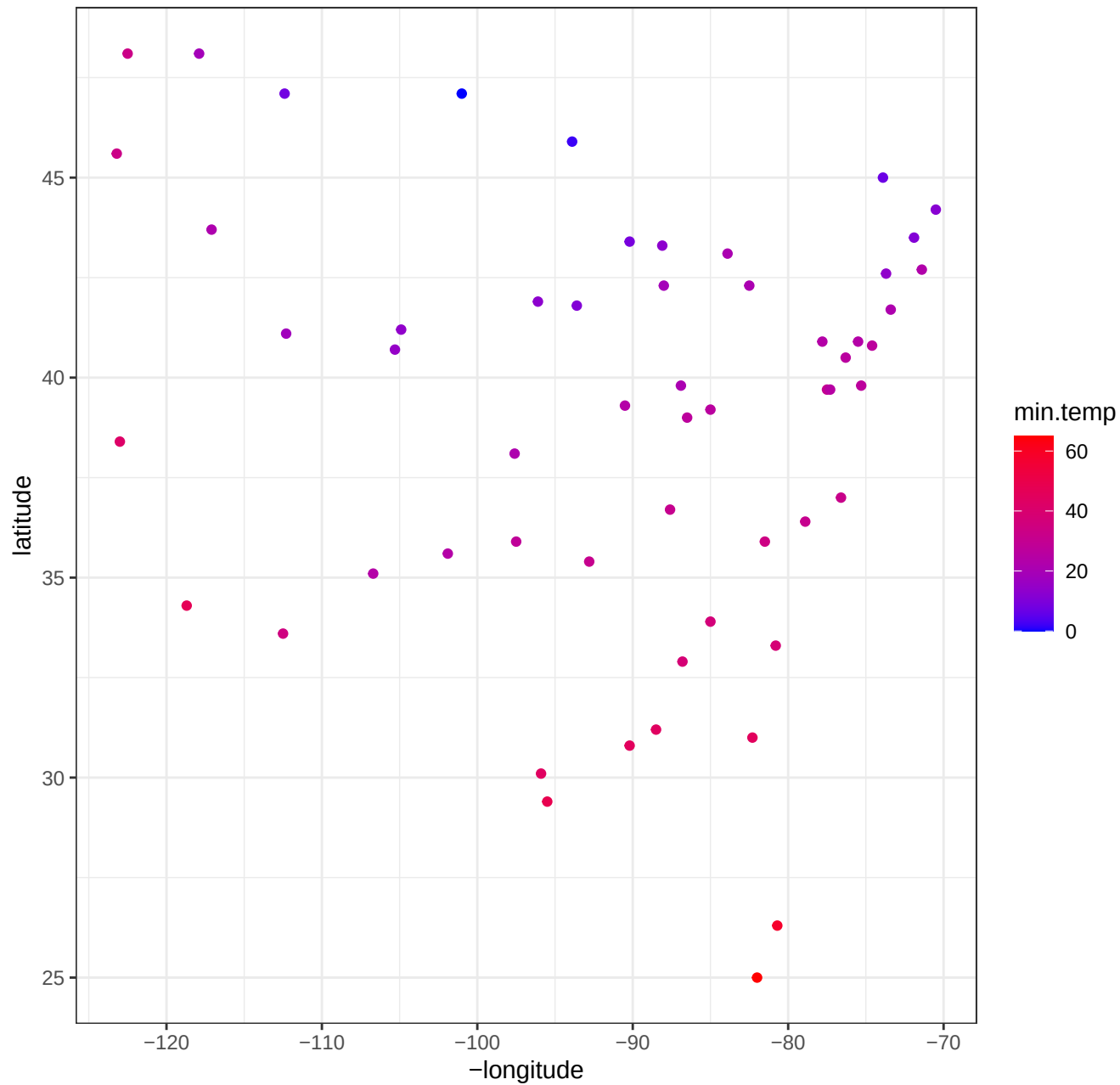
Average minimum temperature in January for some US cities
