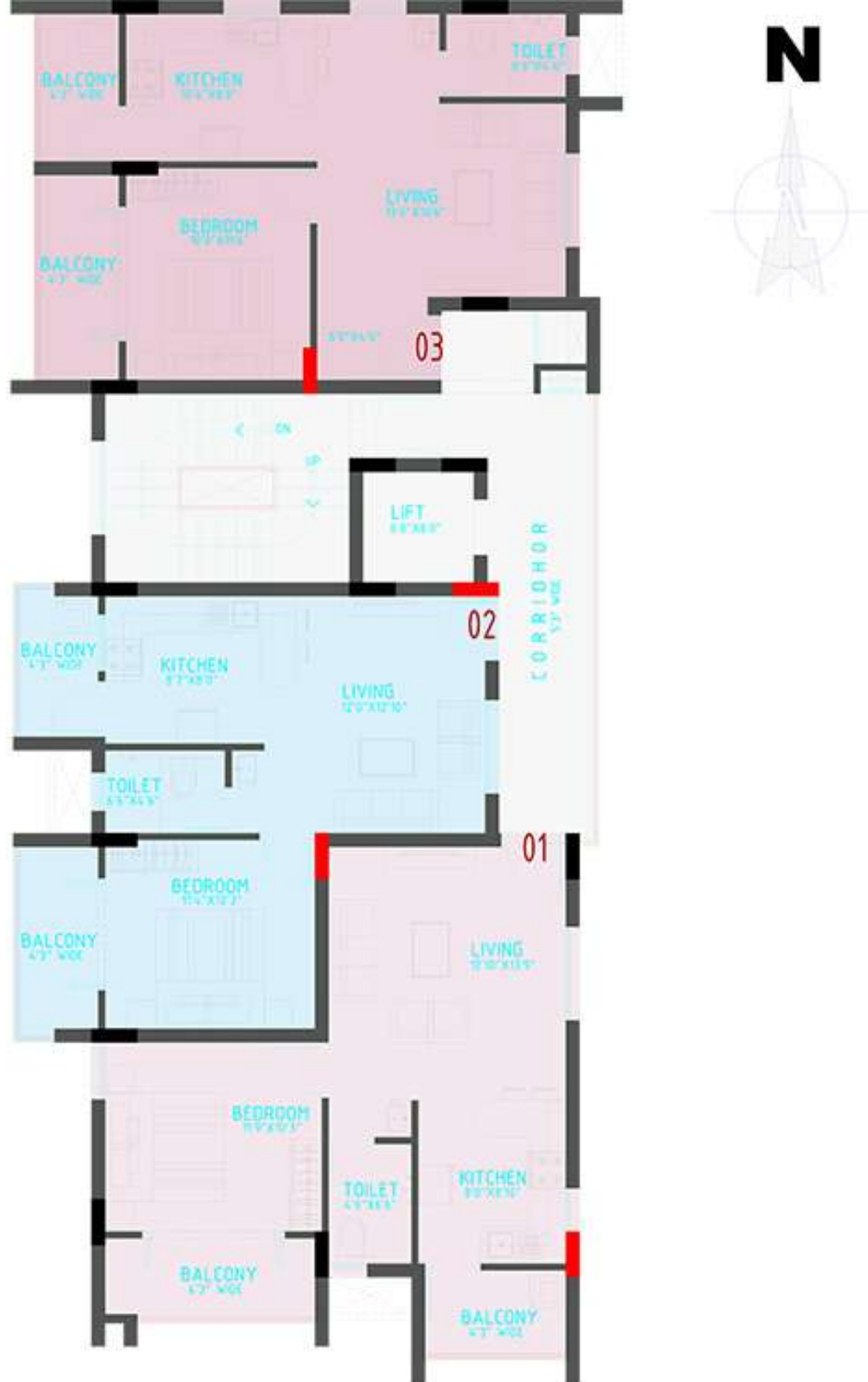
TYPICAL FLOOR PLAN (BLOCK - A)
