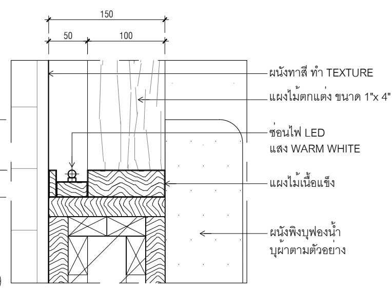
A DETAIL 1 : 5 I-201 BAR - BANQUETTE SEATING
