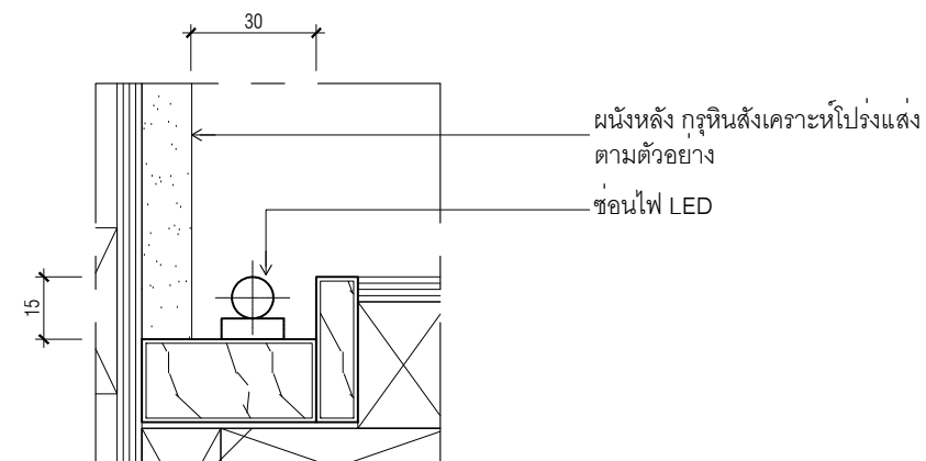
B DETAIL 1 : 2 I-204 COUNTER BAR
