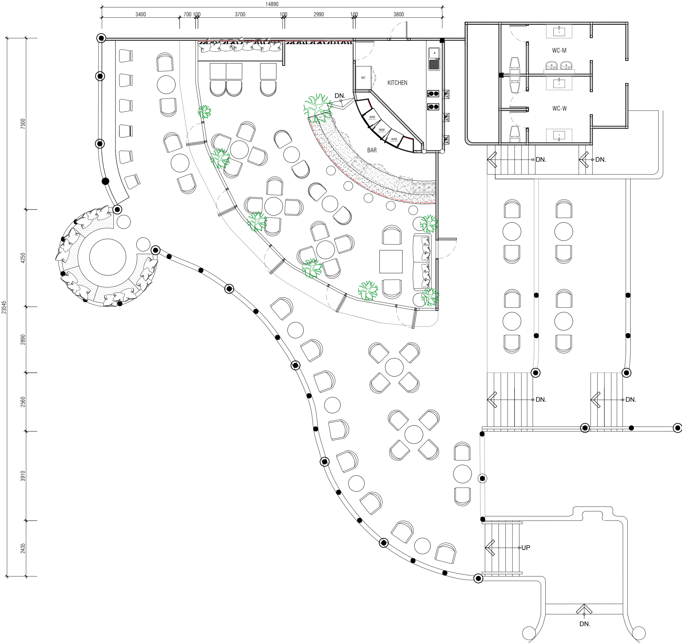
FURNITURE LAYOUT PLAN 1 : 100 SUNSETBAR
