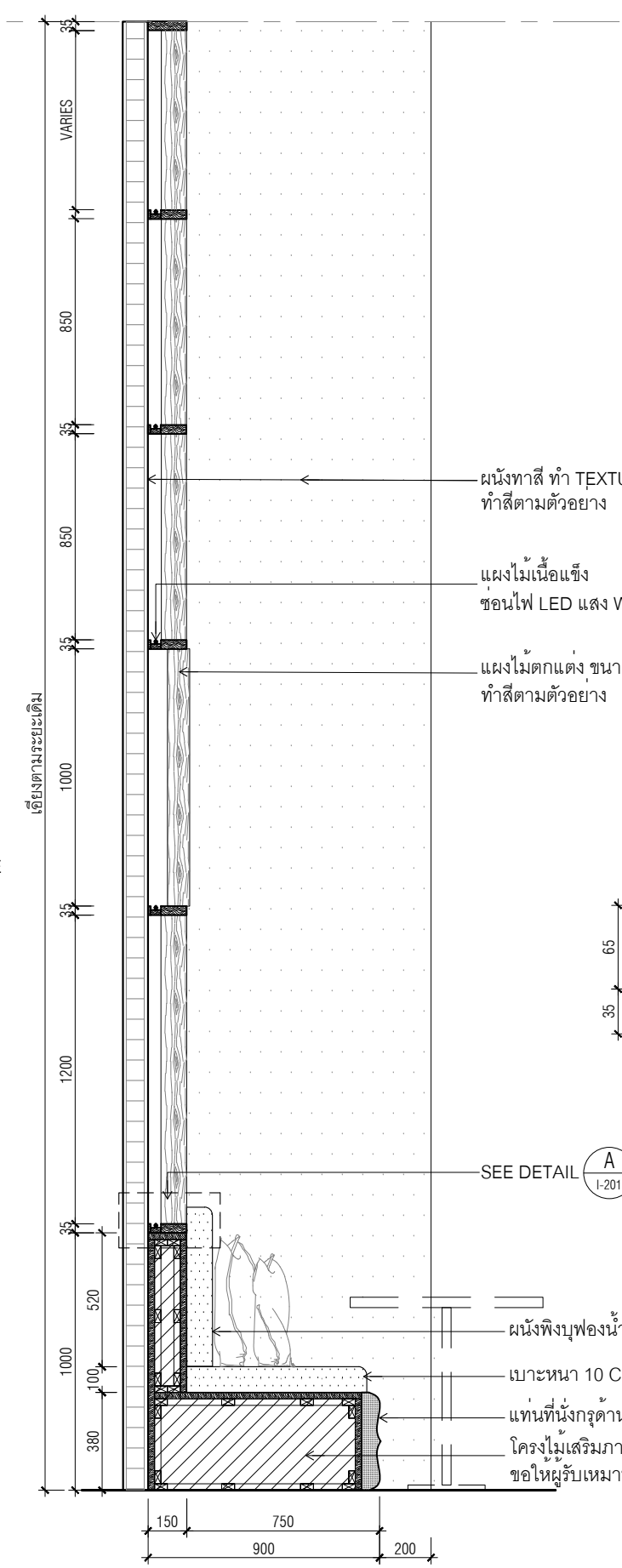
S01 SECTION 1 : 25 I-201 BAR - BANQUETTE SEATING
