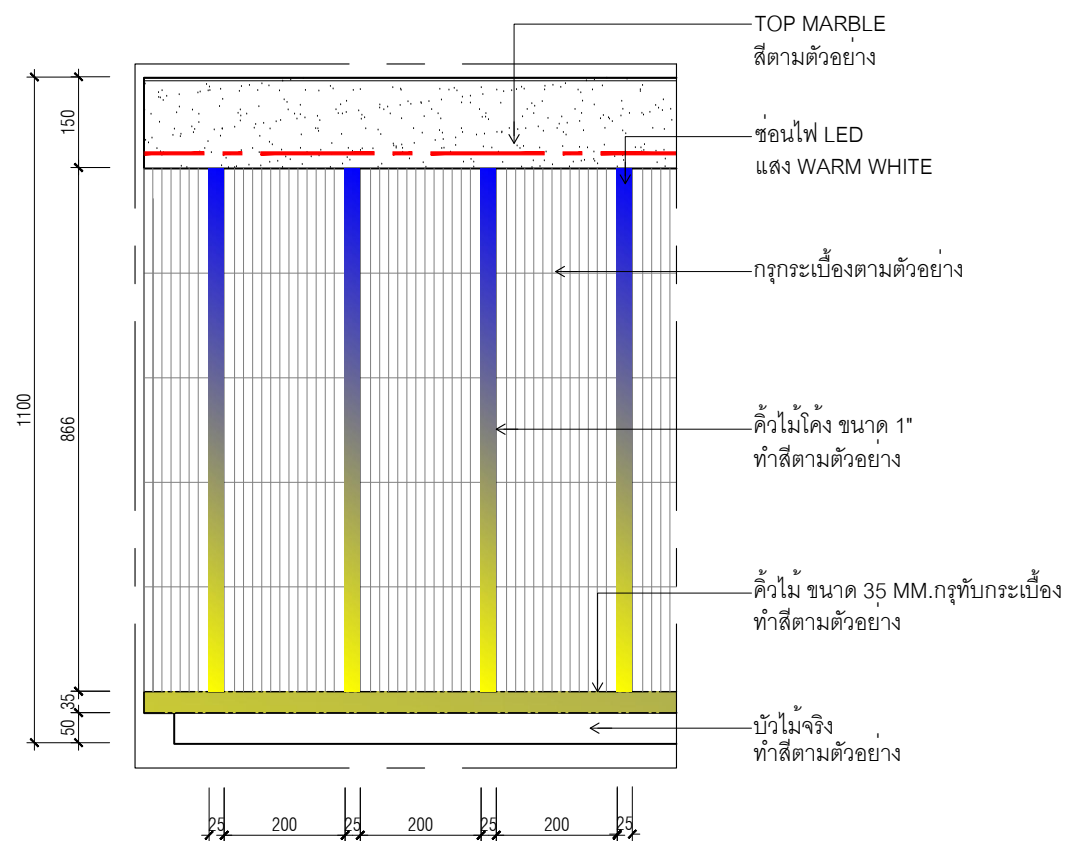
DETAIL A 1 : 12.5
