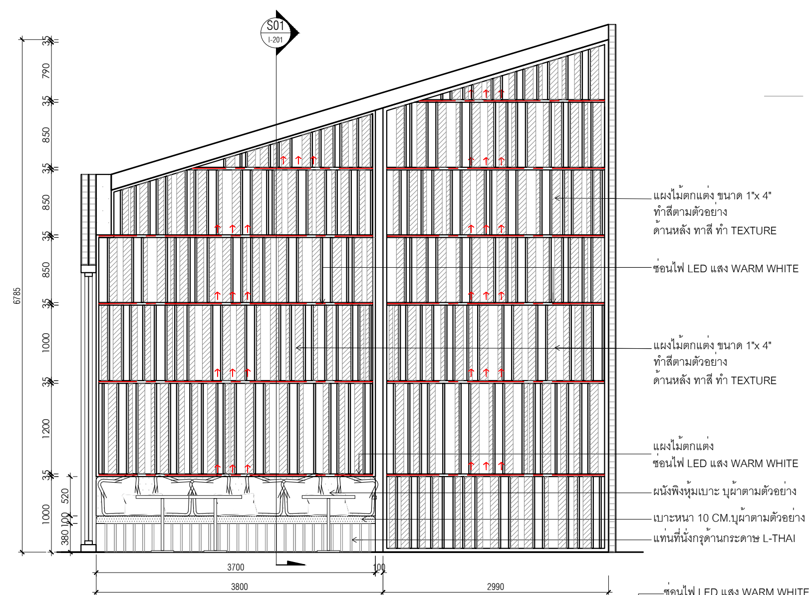
E01 ELEVATION 1 : 50 I-200 BAR - BANQUETTE SEATING
