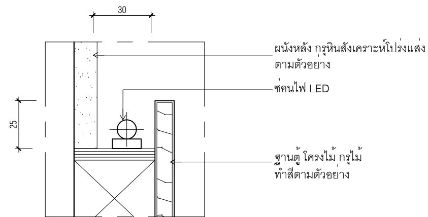
A DETAIL 1 : 2 I-204 COUNTER BAR
