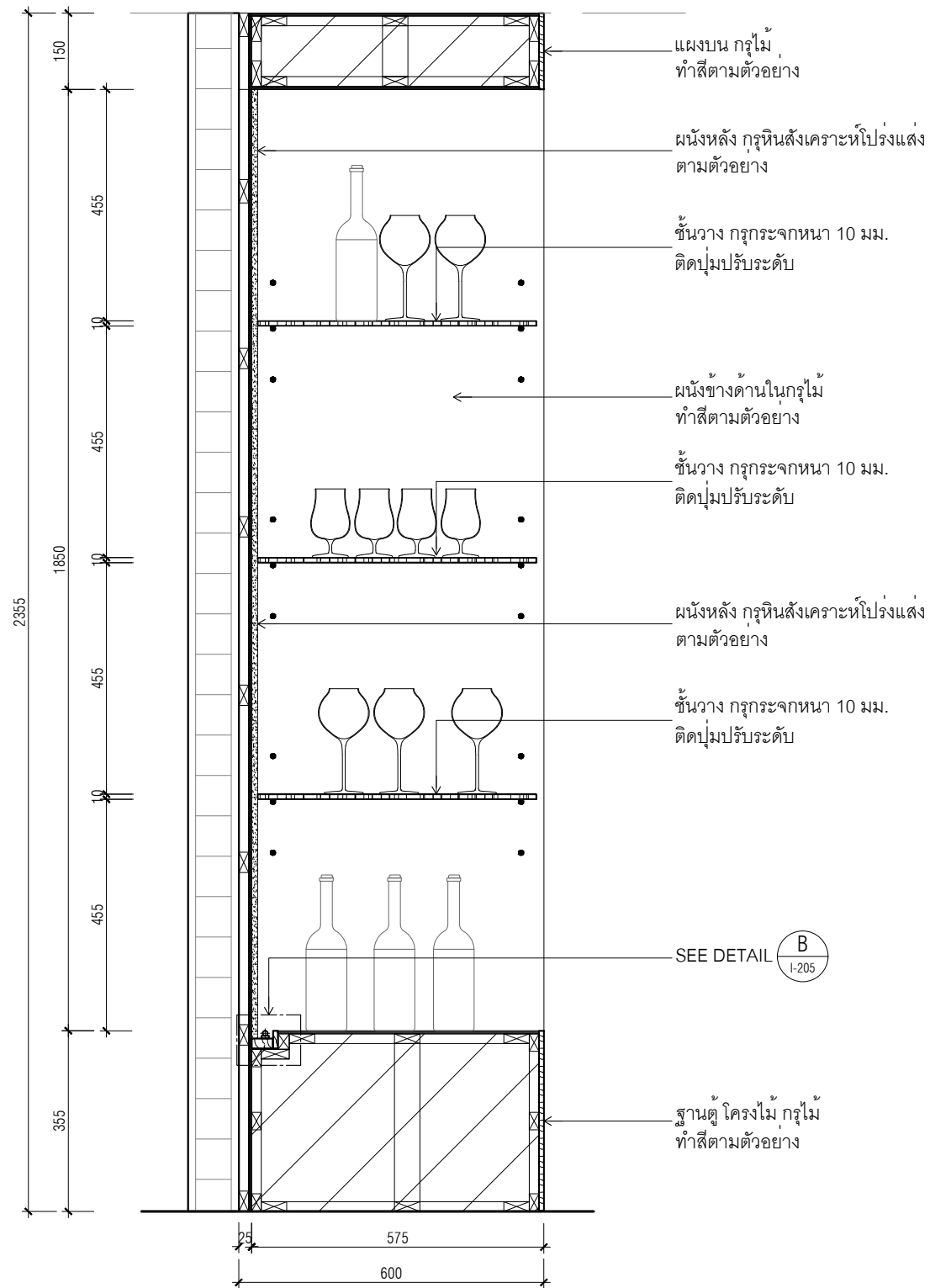
S02 SECTION 1 : 12.5 I-204 COUNTER BAR
