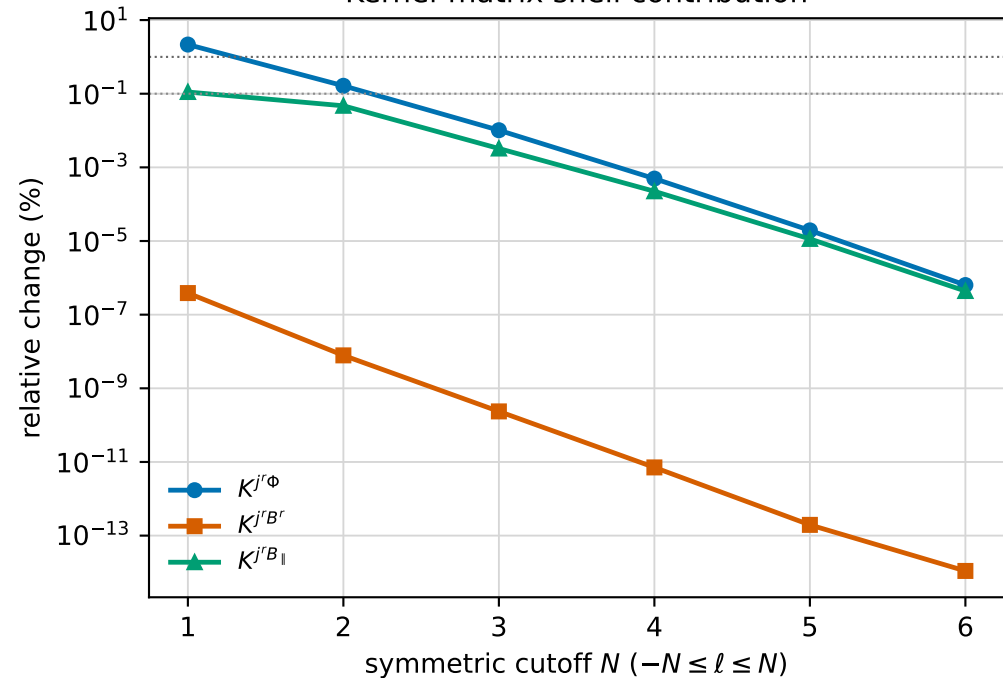
Kernel-matrix shell contribution
