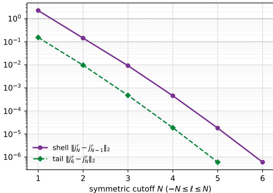
Reconstructed radial-current convergence
