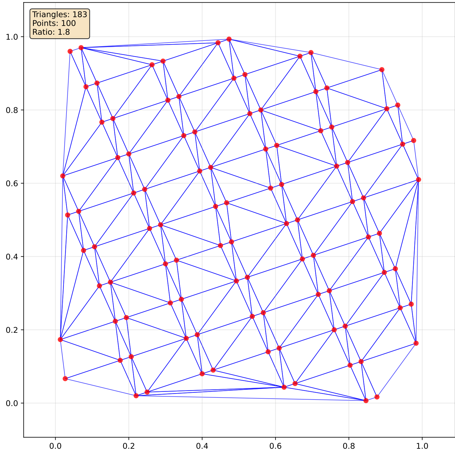
100 Random Points 100 points, 183 triangles
