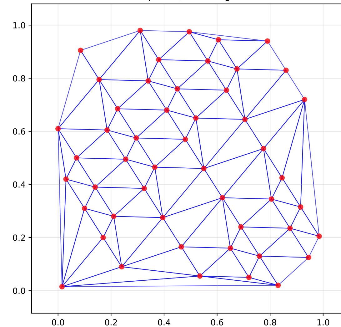
50 Random Points 50 points, 87 triangles
