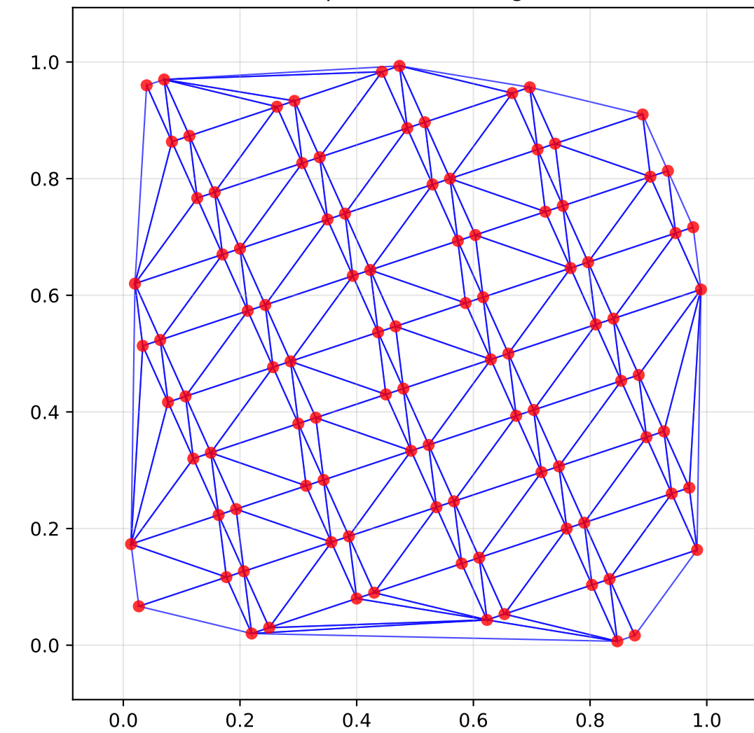
100 Random Points 100 points, 183 triangles
