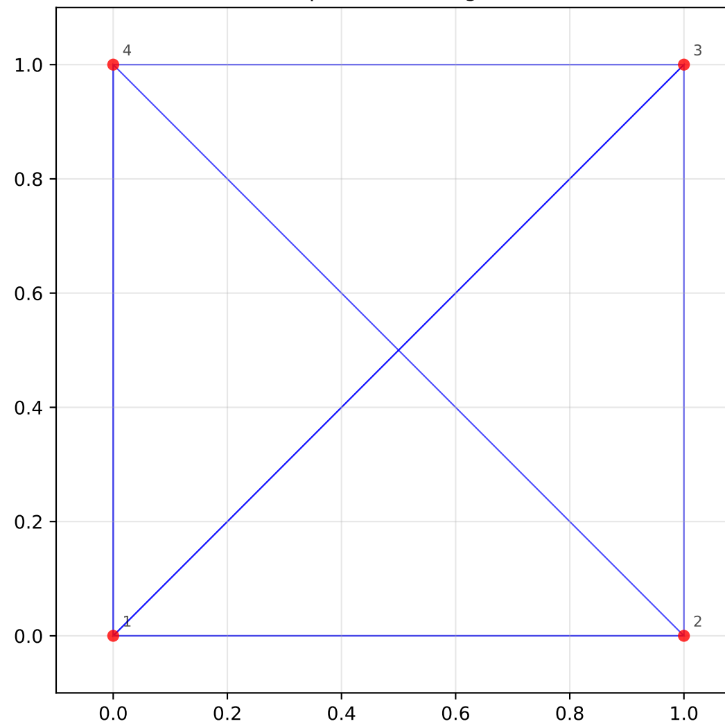
Simple Square 4 points, 3 triangles
