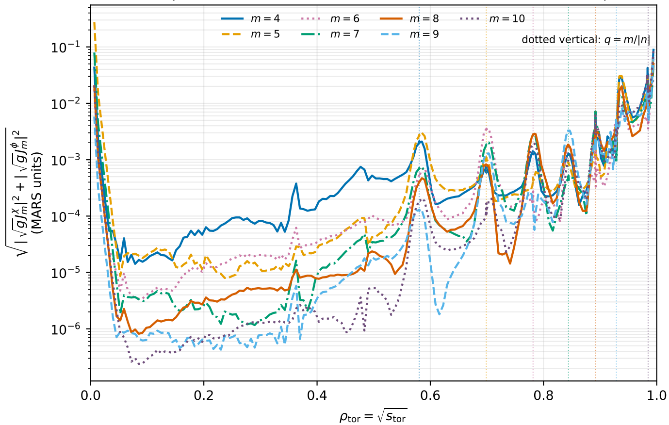
Plasma-response current at n=-3 rational harmonics — ITER TC24 phil000
