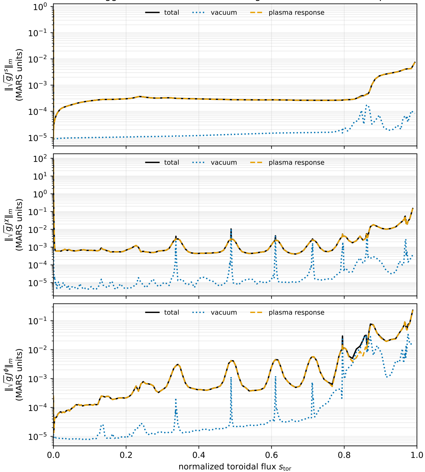
Native-staggered current from MARS magnetic field — ITER TC24 phil000
