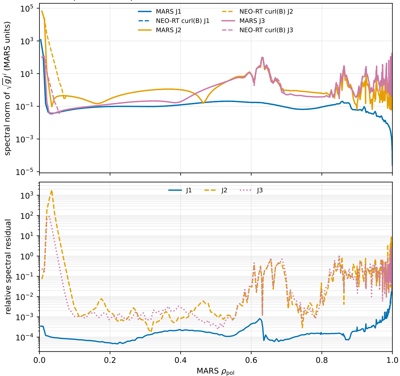
Independent Ampère reconstruction of MARS current — MAST-U Pair A
