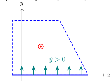
1) Linea y = 0 (Asse x )
