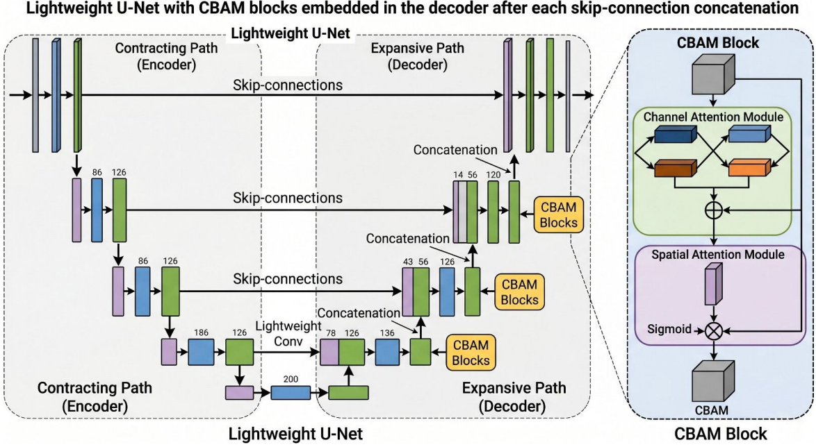
Fig. 1. A schematic diagram illustrating the Lightweight U-Net with CBAM blocks embedded in the decoder after each skip-connection concatenation.
