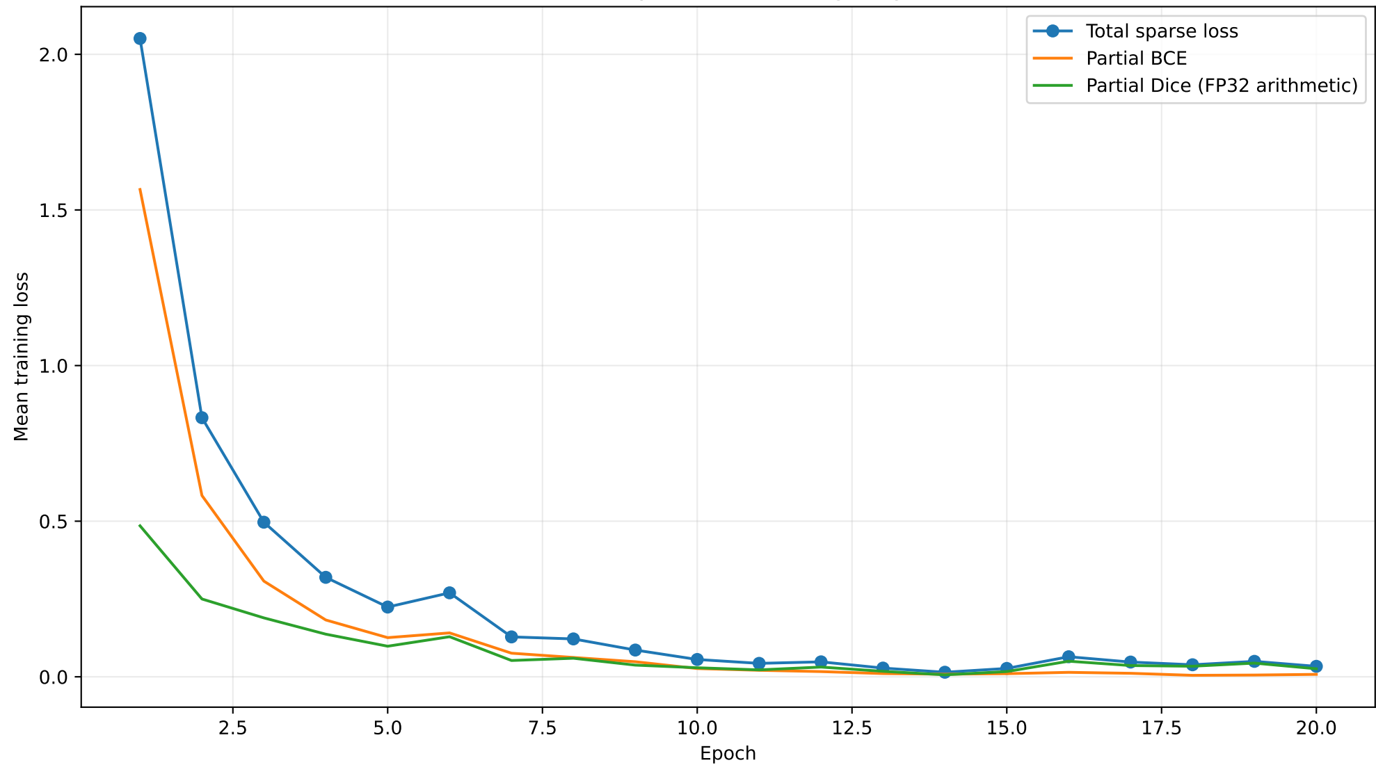
COVA-3D Sanity Fit R2 — Training Diagnostics
